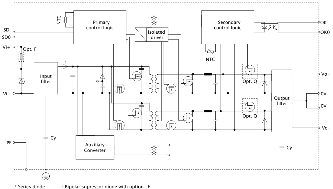
Fig. 1 Block diagram
