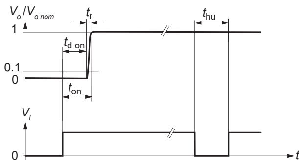
Fig. 7 Typical output response to V_i If option M is not fitted, t_{hu} = 0 ms.
