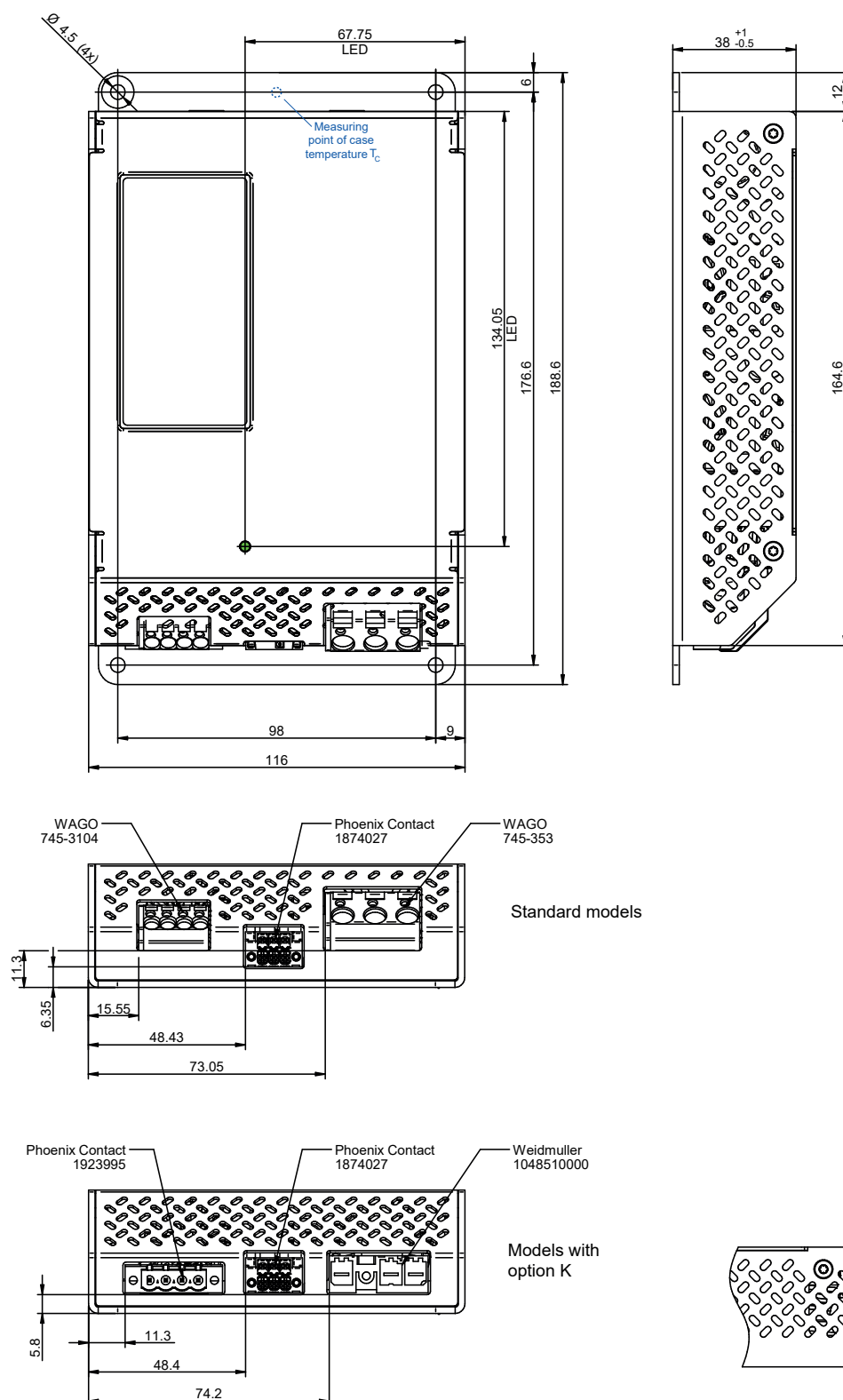
Fig. 8 Case of RCM200/300 (RCM02) weight approx. 820 g, Aluminum, EP-powder coated
