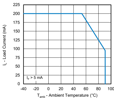
Fig. 5 Load Current vs. Ambient Temperature
