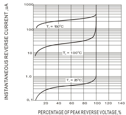
Fig.4-TYPICAL REVERSE CHARACTERISTIC
