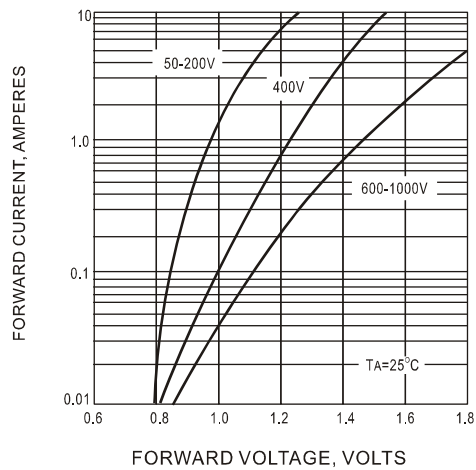
Fig.3 FORWARD CHARACTERISTICS
