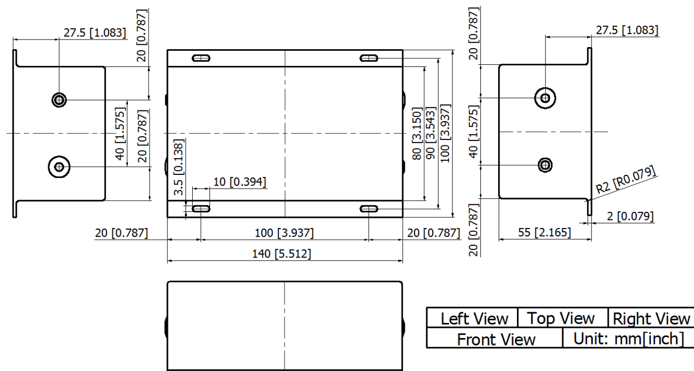
Figure 14. Outline Dimensions
