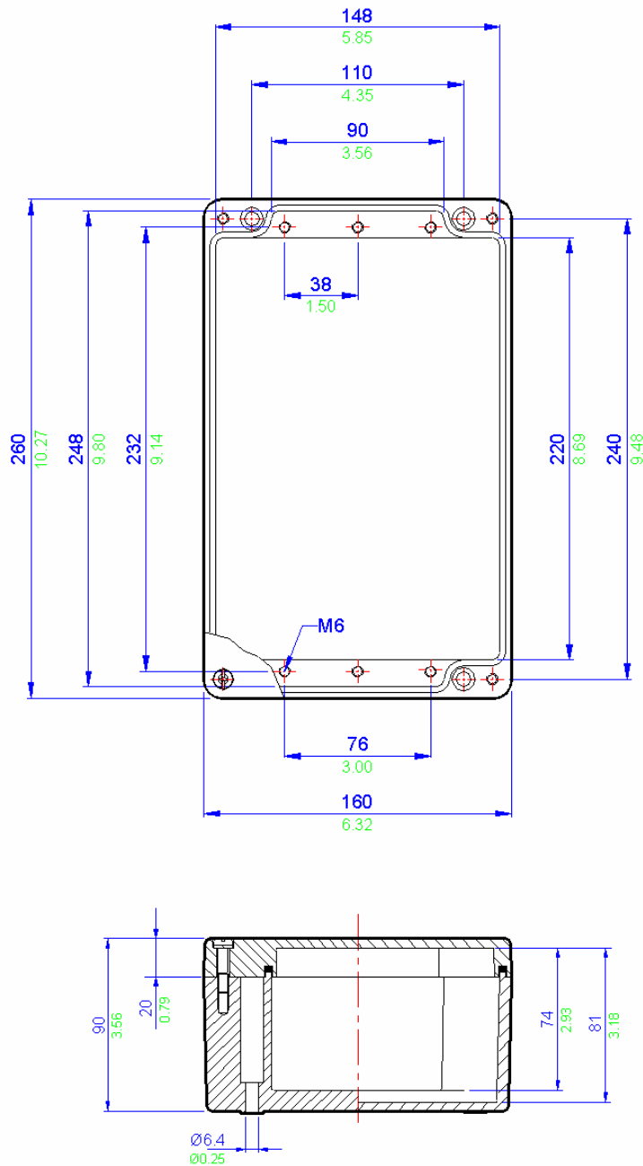
BPG 9 / BPGC 9 Drawing
