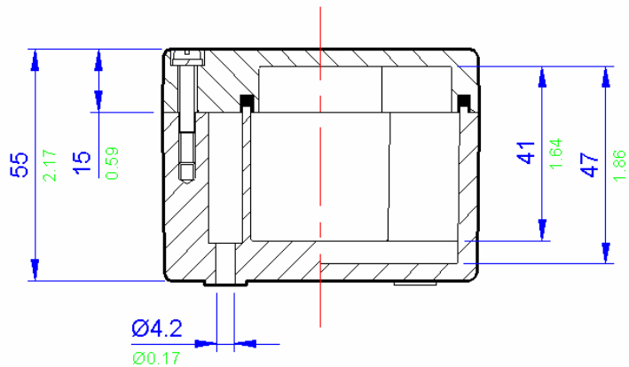
BPG 2 / BPGC 2 Drawing
