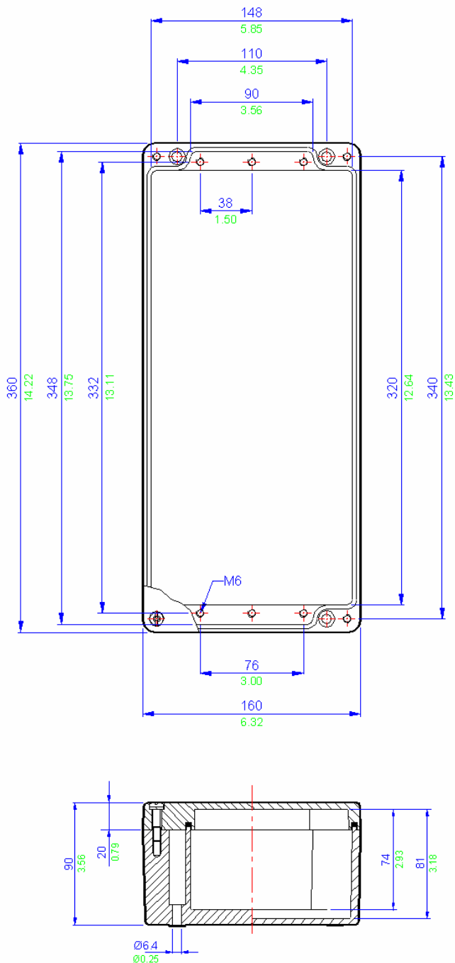
BPG 10 / BPGC 10 Drawing
