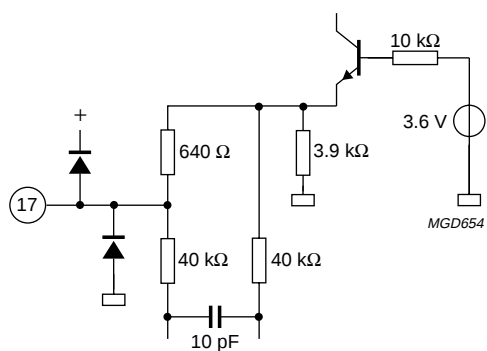
Fig.27 Pin 17; V_{iFM} .
