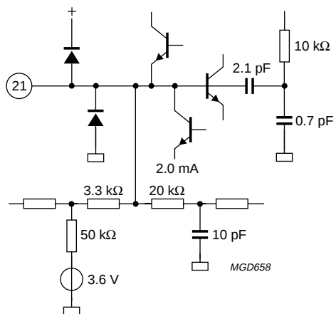
Fig.31 Pin 21; V_{o(vid)} .
