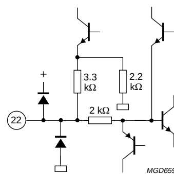
Fig.32 Pin 22; V_{i(vid)} .
