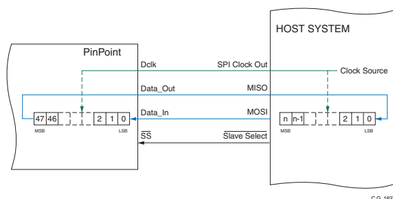
Figure 7.5 SPI® Data Transfer Principle
