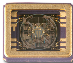
Figure 13.2 CRM100 (Lid Removed)
