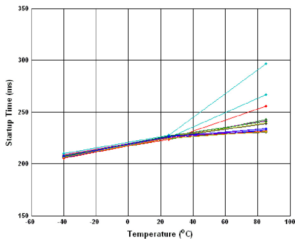
Figure 5.48 Startup Time vs Temperature (Vdd = 2.7V)
