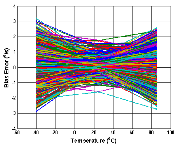
Figure 5.2 Analogue Bias Error (dsp) vs Temperature
