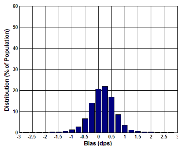
Figure 5.16 Analogue Bias (dps) at -40°C
