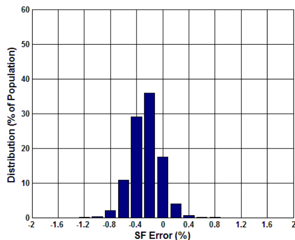
Figure 5.19 Analogue SF Error (%) Over Temperature
