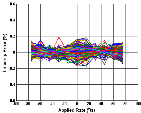
Figure 5.30 Digital NL Error (%) vs Applied Rate (-40°C)
