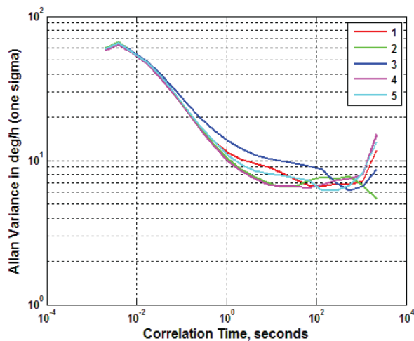
Figure 5.52 Allan Variance of CRM100s 75°/s 25Hz
