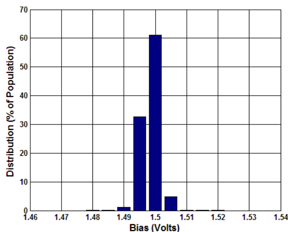
Figure 5.14 Analogue Bias at 25°C
