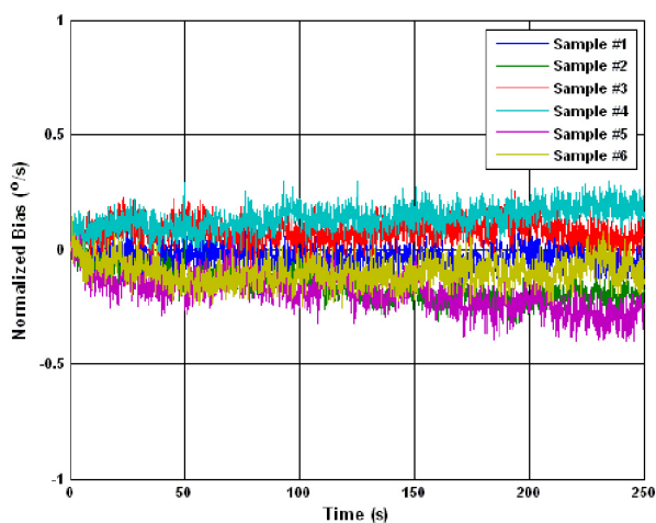
Figure 5.50 Normalised Bias Drift after Switch-On
