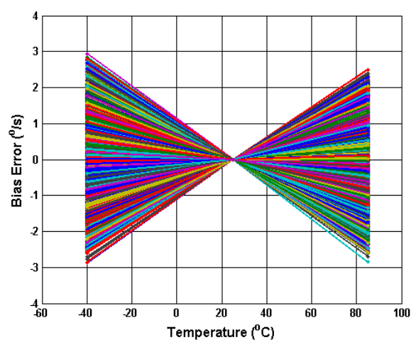
Figure 5.3 Analogue Normalised Bias Error (dps) vs Temperature
