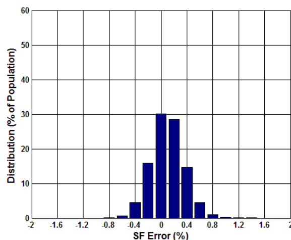
Figure 5.39 Digital SF Error (%) over Temperature
