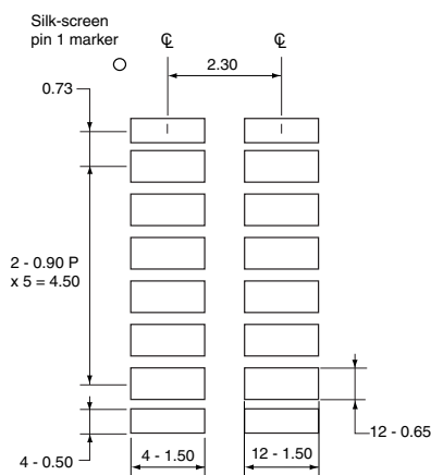
Figure 7.2 Recommended Pad Layout (CRM200)
