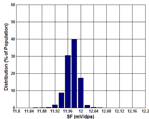
Figure 5.20 Analogue SF at 25°C
