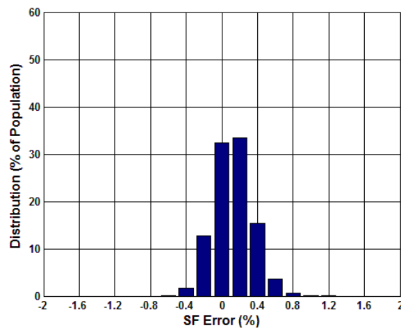
Figure 5.40 Digital SF Error (%) at 25°C
