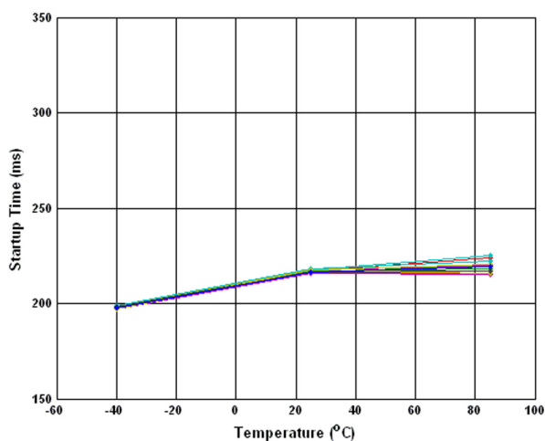
Figure 5.49 Startup Time vs Temperature (Vdd = 3.6V)
