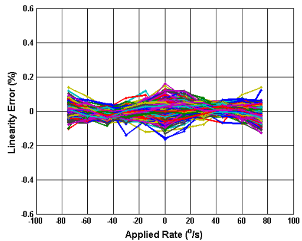
Figure 5.31 Digital NL Error (%) vs Applied Rate (25°C)
