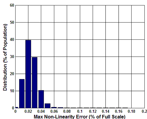
Figure 5.23 Analogue Maximum Linear Error (%) at 25°C
