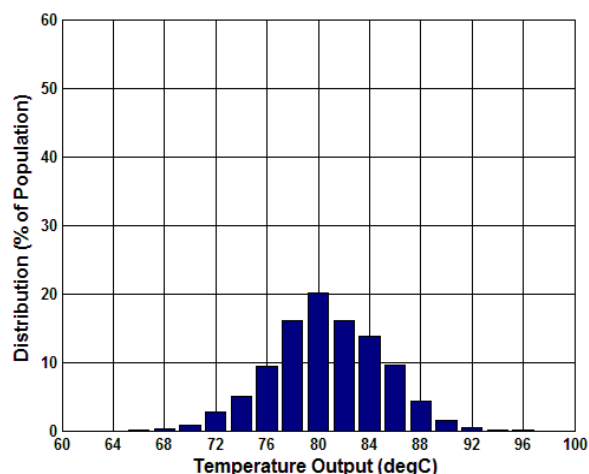
Figure 5.47 Temperature Output (°C) at 85°C
