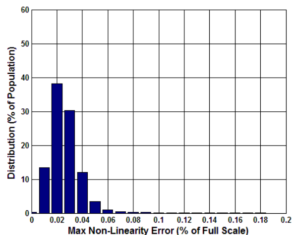
Figure 5.22 Analogue Maximum Linear Error (%) at -40°C
