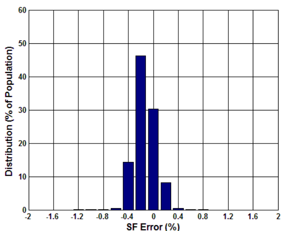
Figure 5.41 Digital Normalised SF Error (%) over Temperature
