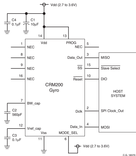
Figure 7.4 Peripheral Circuit - Digital Output (CRM200)
