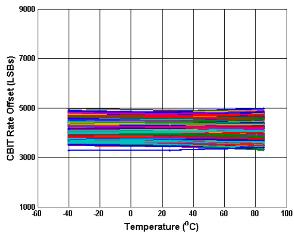
Figure 5.34 Digital CBIT (LSB) vs Temperature
