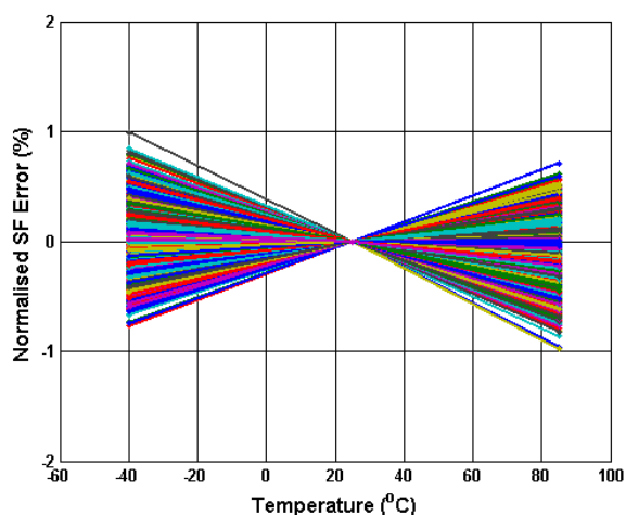
Figure 5.6 Analogue Normalised Scale Factor Error (%) vs Temperature
