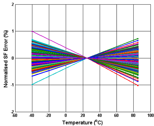
Figure 5.29 Digital Normalised Error (%) vs Temperature
