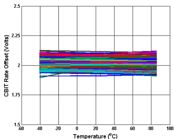
Figure 5.11 Analogue CBIT Offset (Volts) vs Temperature
