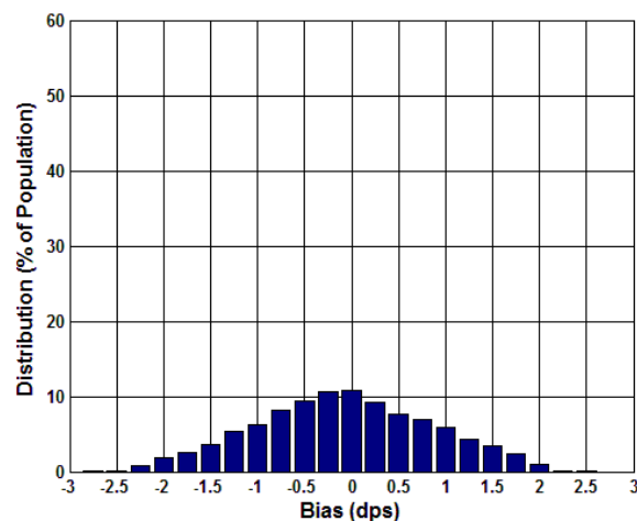
Figure 5.18 Analogue Bias (dps) at 85°C
