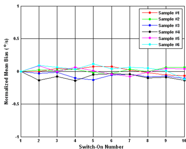
Figure 5.51 Switch-On Repeatability of Normalised Mean Bias
