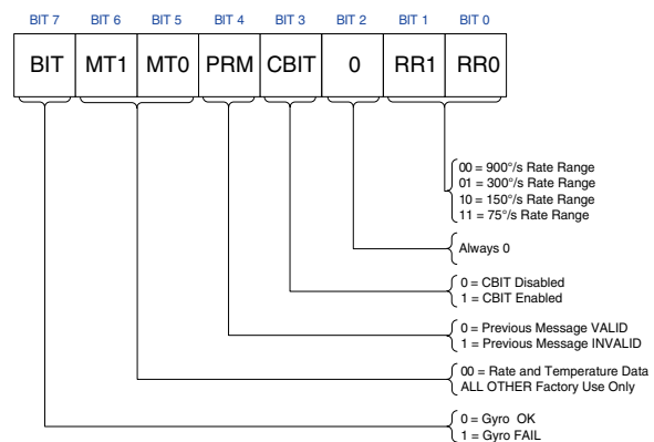
Figure 7.10 Status Byte Format
