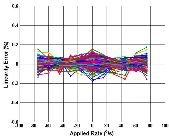
Figure 5.9 Analogue NL Error (%) vs Applied Rate (25°C)
