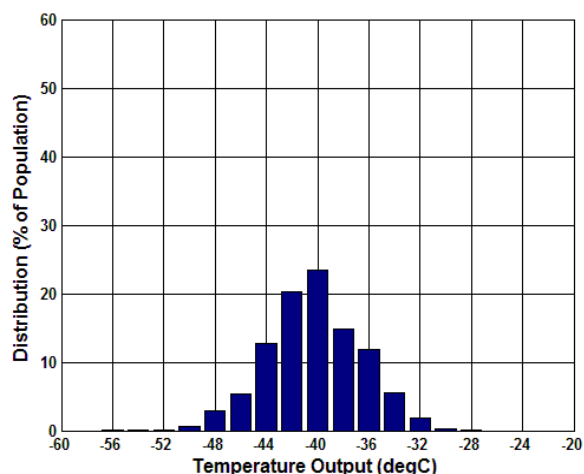
Figure 5.45 Temperature Output (°C) at -40°C
