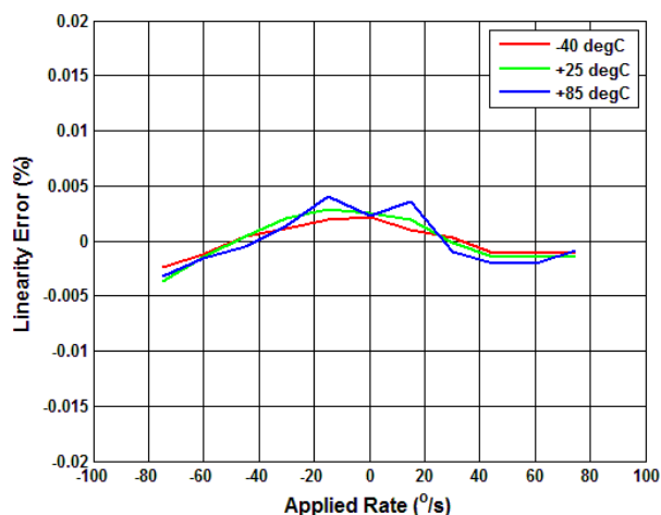
Figure 5.7 Analogue Ave NL Error (%) vs Applied Rate
