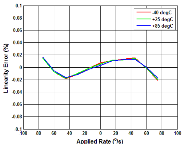
Figure 5.33 Digital Ave Error (%) vs Applied Rate
