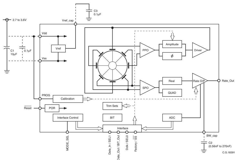
Figure 1.1 CRM200 Functional Block Diagram
