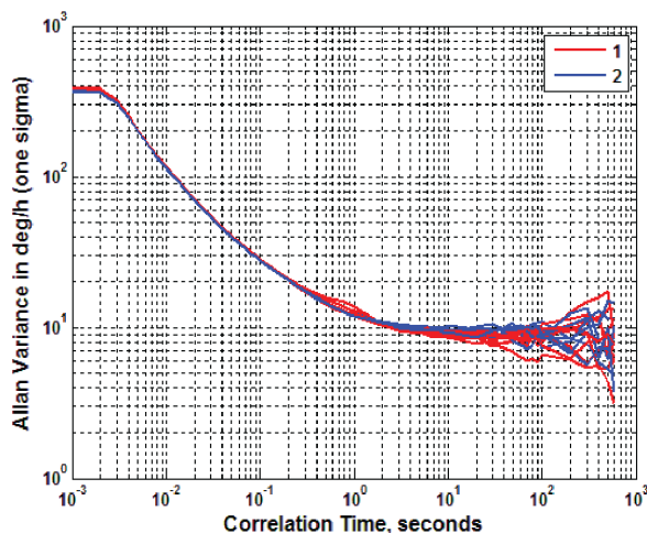
Figure 5.53 Allan Variance of CRM100s 900°/s 150Hz
