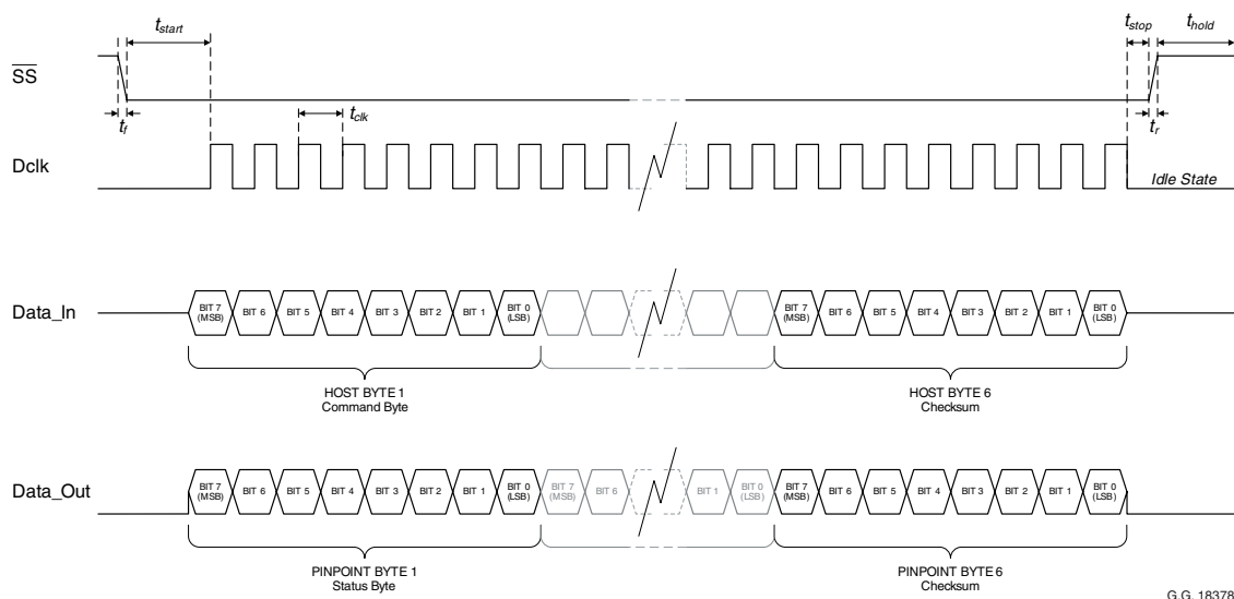
Figure 7.6 SPI® Timing
