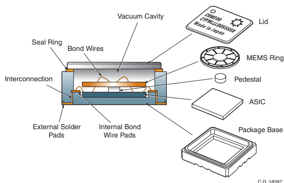
Figure 13.1 CRM100 Main Components
