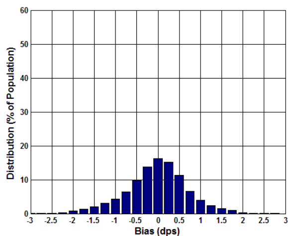
Figure 5.38 Digital Normalised Bias Distribution (dps) over Temperature
