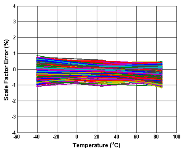
Figure 5.5 Analogue Scale Factor Error (%) vs Temperature
