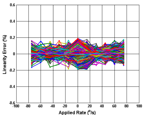
Figure 5.10 Analogue NL Error (%) vs Applied Rate (85°C)
