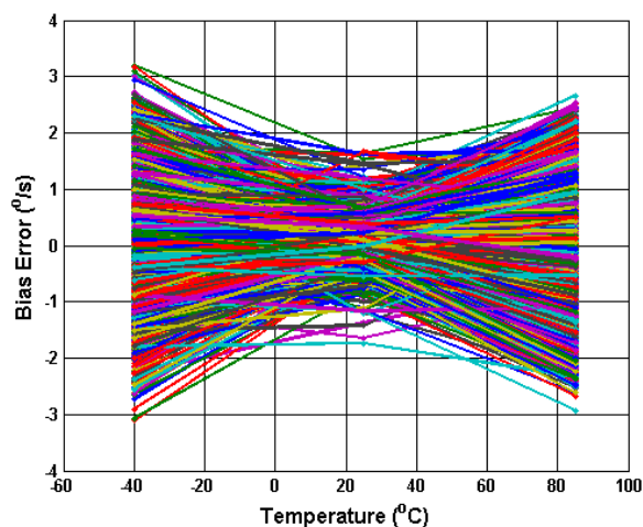
Figure 5.25 Digital Bias Error (dps) vs Temperature
