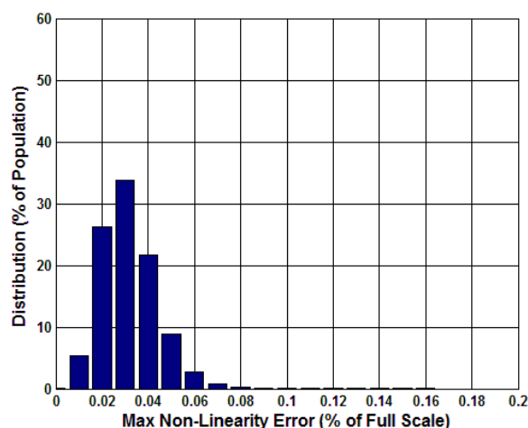
Figure 5.43 Digital Maximum Linear Error (%) at 25°C
