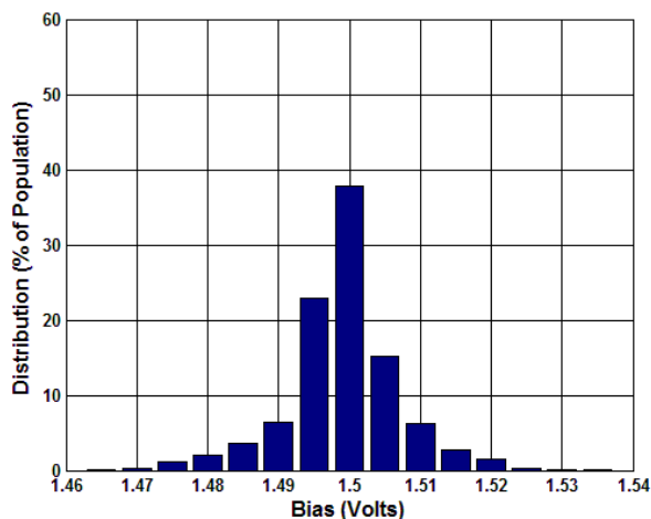
Figure 5.13 Analogue Bias (Volts) Over Temperature
