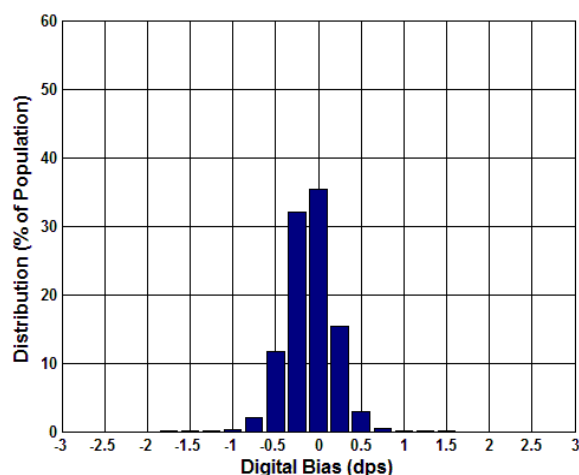
Figure 5.37 Digital Bias (dps) at 25°C
