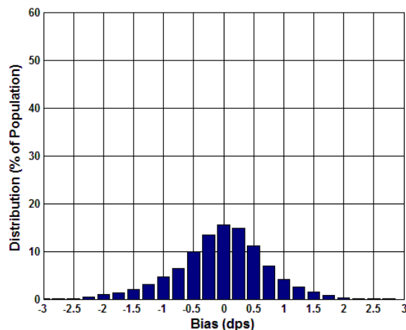
Figure 5.15 Analogue Normalised Bias Distribution (dps) Over Temperature
