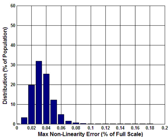
Figure 5.42 Digital Maximum Linear Error (%) at -40°C
