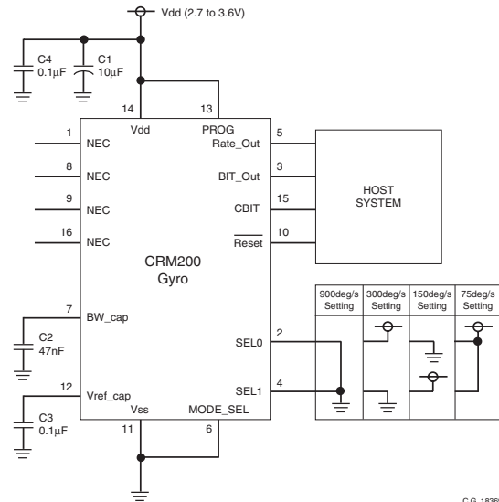
Figure 7.3 Peripheral Circuit - Analogue Output (CRM200)
