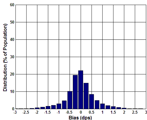
Figure 5.36 Digital Bias Distribution (dps) over Temperature
