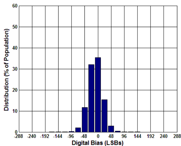
Figure 5.35 Digital Bias (LSB) at 25°C
