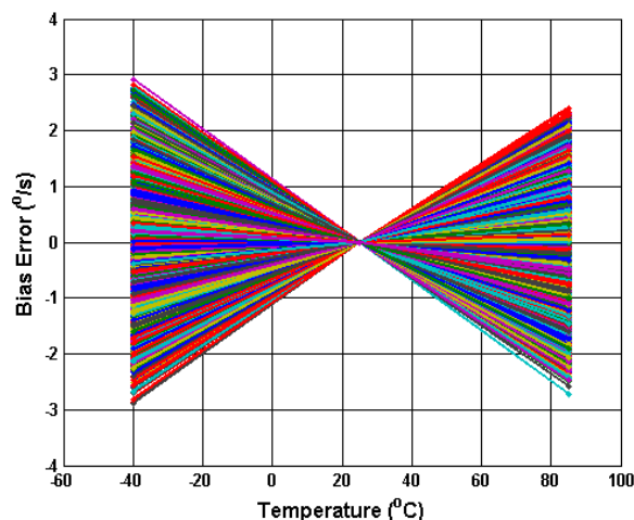
Figure 5.26 Digital Normalised Bias Error (dps) vs Temperature
