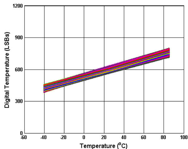
Figure 5.27 Digital Temperature Output (LSB) vs Temperature
