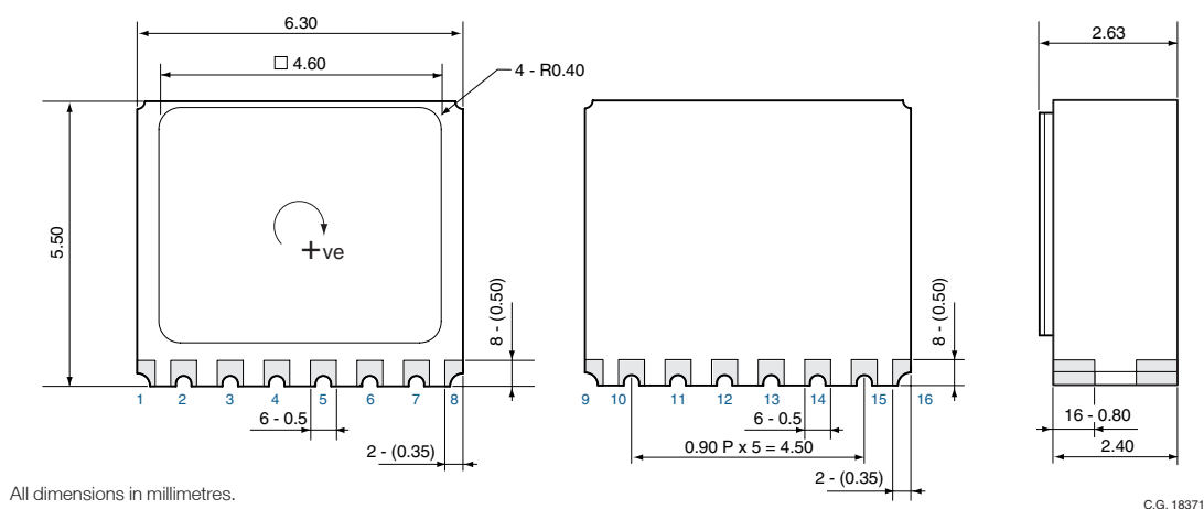
Figure 1.2 CRM200 Overall Dimensions
