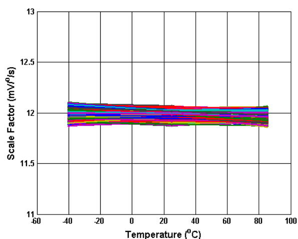
Figure 5.4 Analogue Scale Factor vs Temperature
