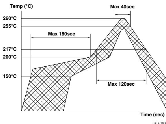
Figure 10.1 Recommended Reflow Solder Profile
