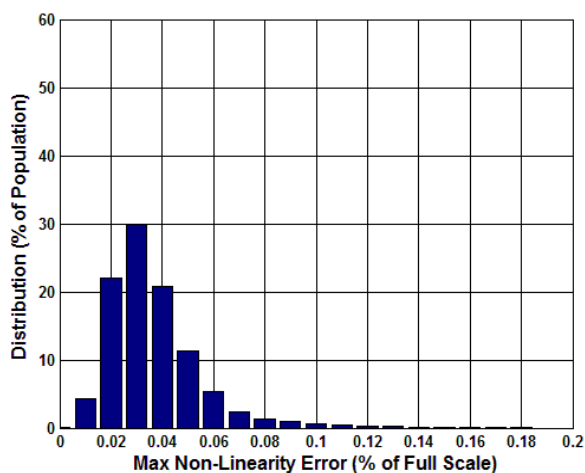
Figure 5.44 Digital Maximum Linear Error (%) at 85°C
