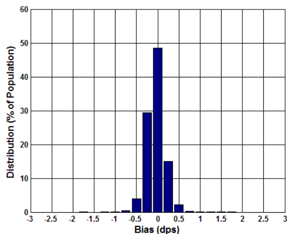
Figure 5.17 Analogue Bias (dps) at 25°C
