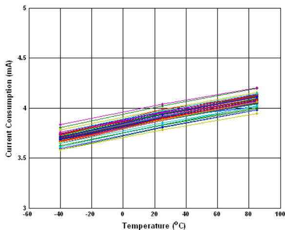
Figure 5.12 Current Consumption vs Temperature
