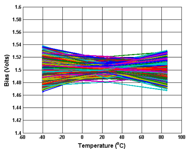
Figure 5.1 Analogue Bias (Volts) vs Temperature
