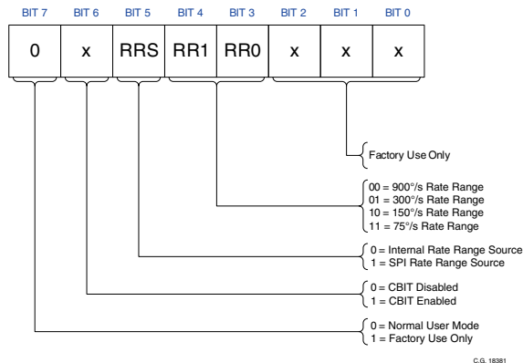
Figure 7.9 Command Byte Format
