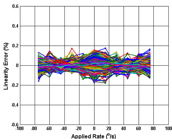
Figure 5.8 Analogue NL Error (%) vs Applied Rate (-40°C)
