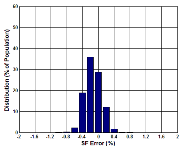
Figure 5.21 Analogue Normalised SF Error (%) Over Temperature
