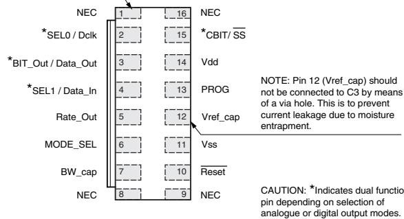
Figure 7.1 Pinout (CRM200) (Top View)
