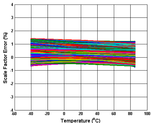
Figure 5.28 Digital Scale Factor Error (%) vs Temperature
