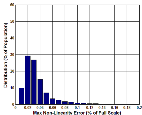
Figure 5.24 Analogue Maximum Linear Error (%) at 85°C
