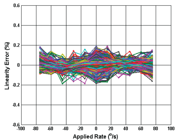
Figure 5.32 Digital NL Error (%) vs Applied Rate (85°C)
