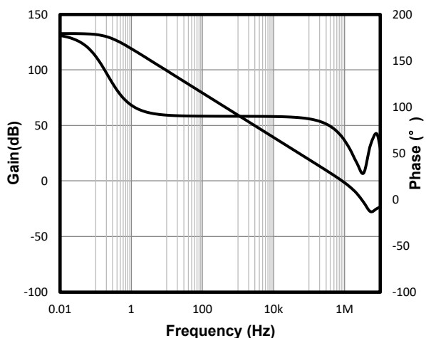
Figure 7. Open-Loop Gain and Phase vs. Frequency
