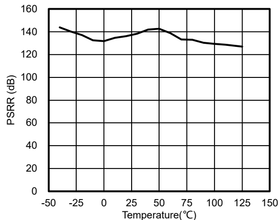
Figure 10. PSRR vs. Temperature
