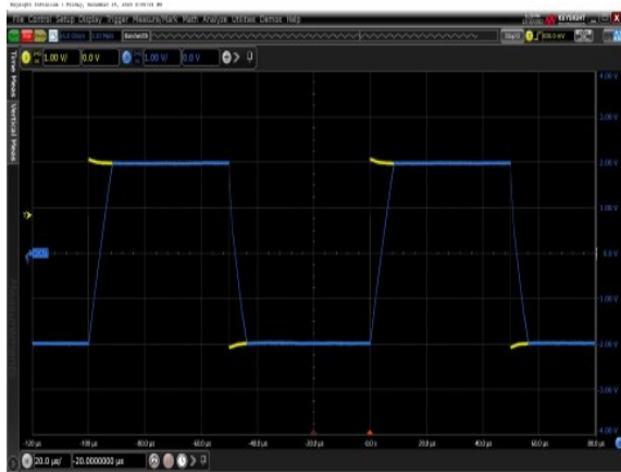
Figure 15. Large-Signal Response, 4-V Step, G = 1
