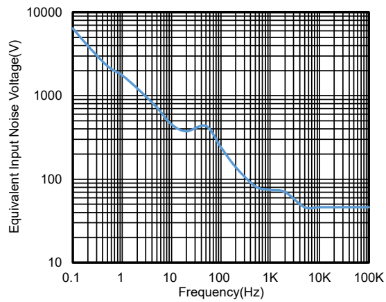
Figure 13. Voltage Noise Spectral Density vs. Frequency
