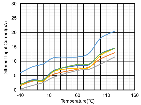
Figure 14. Different Input Current vs. Temperature
