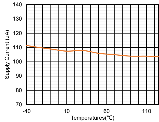
Figure 2. Quiescent Current vs. Temperature
