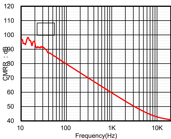
Figure 11. CMRR vs. Frequency
