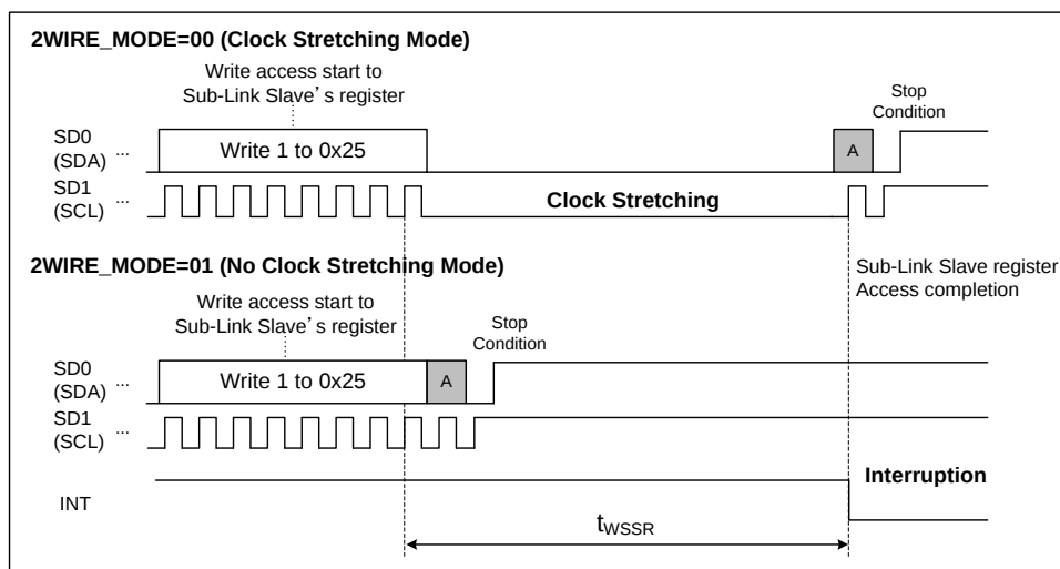
Figure 29. Write access completion time to Sub-Link Slave register
