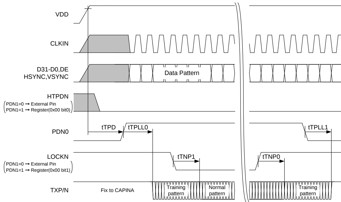
Figure 26. THCV235-Q Lock/Unlock Sequence
