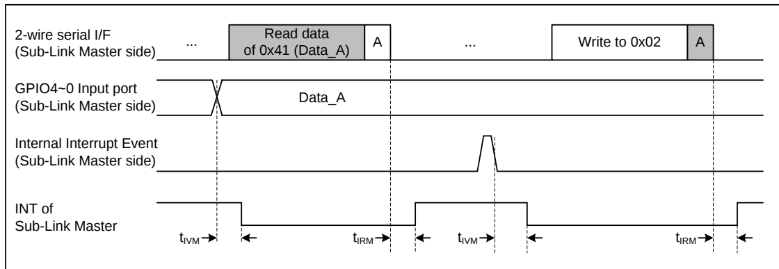
Figure 37. GPIO input and other interrupt event timing at Sub-Link Master side
