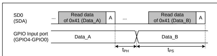
Figure 34. Programmable GPIO input timing at Sub-Link Master side
