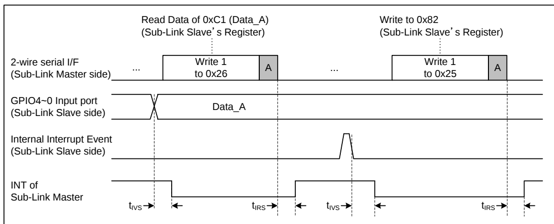
Figure 38. GPIO input and other interrupt event timing at Sub-Link Slave side (Clock Stretching Mode)
