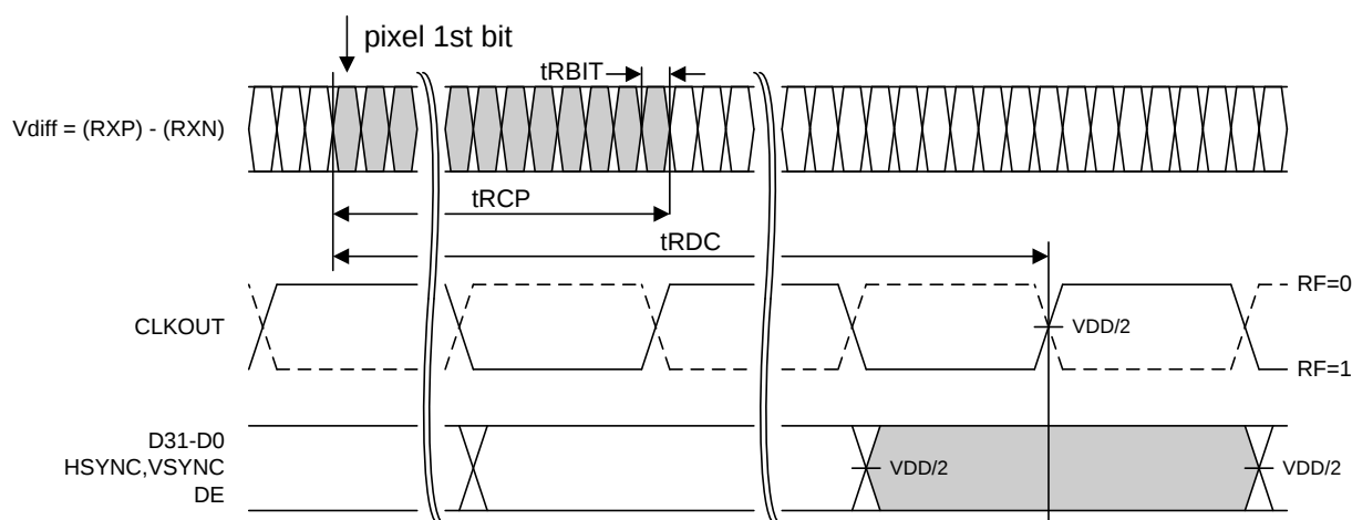
Figure 25. THCV236-Q Latency
