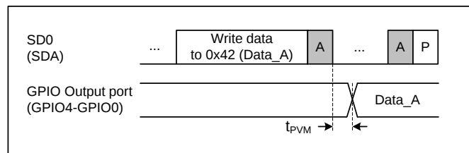
Figure 35. Programmable GPIO output timing at Sub-Link Master side
