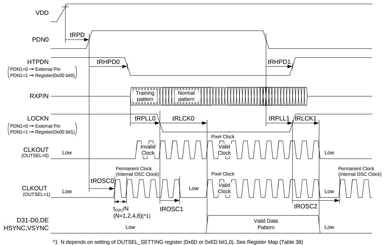
Figure 27. THCV236-Q Lock/Unlock Sequence
