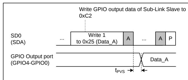
Figure 36. Programmable GPIO output timing at Sub-Link Slave side
