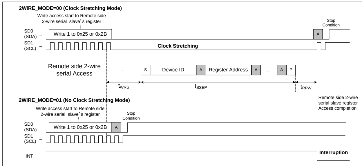
Figure 31. Write access completion time to Remote side 2-wire serial slave register
