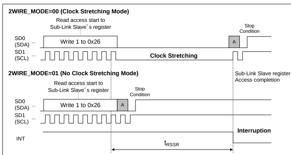
Figure 30. Read access completion time to Sub-Link Slave register
