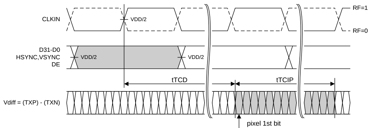
Figure 24. THCV235-Q Latency
