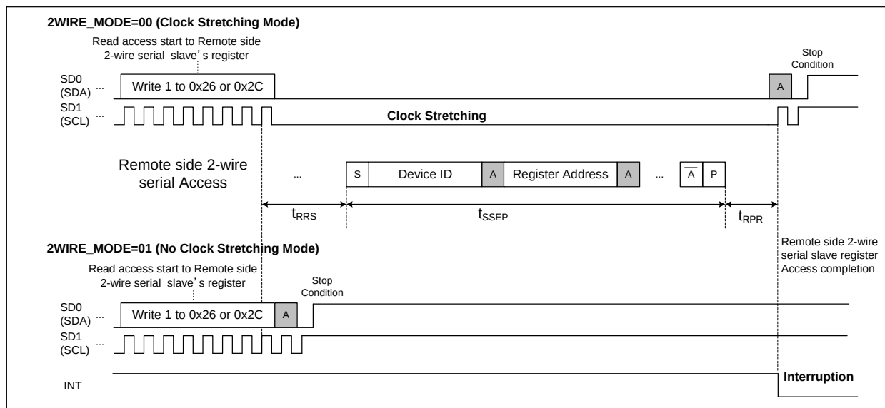
Figure 32. Read access completion time to Remote side 2-wire serial slave register
