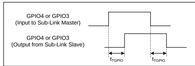
Figure 33. Through GPIO delay
