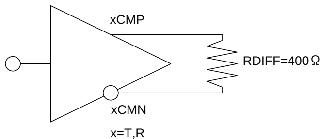
Figure 23. Bi-directional CML VBOD/VBOC Test Circuit
