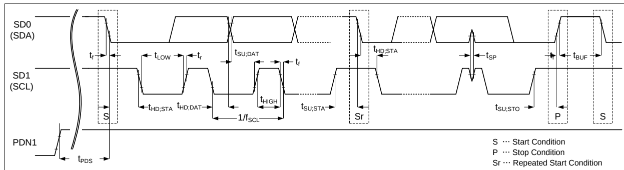
Figure 28. 2-wire serial interface Timing Diagram
