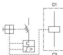
Connection Diagrams RS
