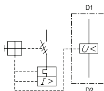
Connection Diagrams RU
