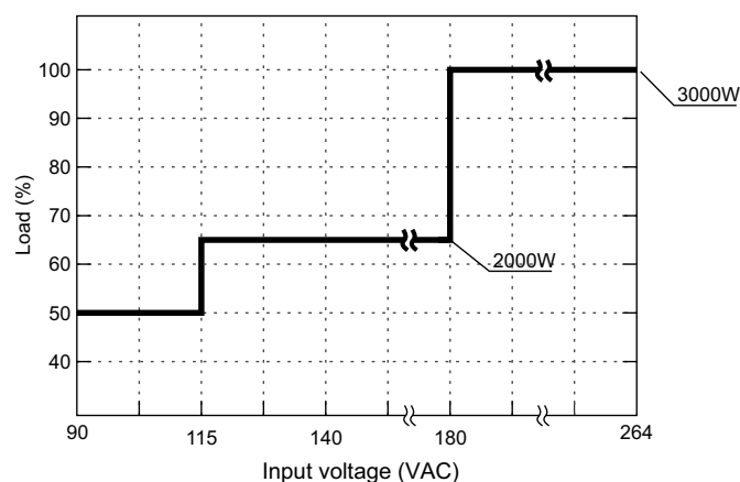
Input derating curve
