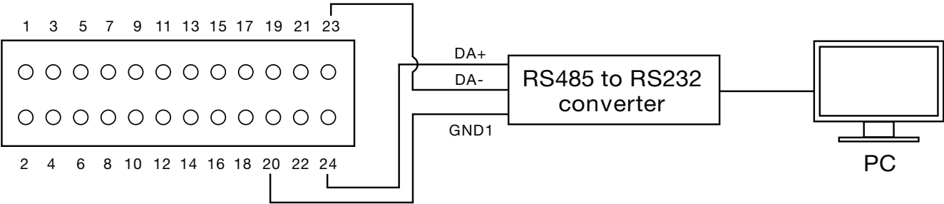
RS232 connection diagram
