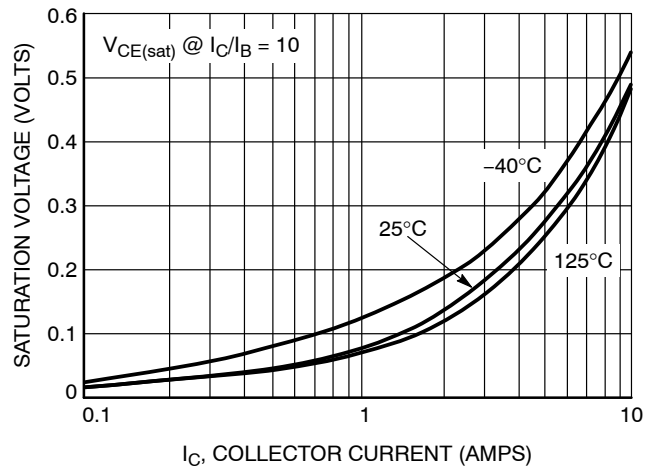
Figure 6. D45H11 ON-Voltage
