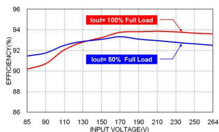
TAD65US24C-P Efficiency VS Input Voltage
