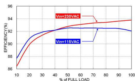
TAD65US24C-P Efficiency VS Output Load
