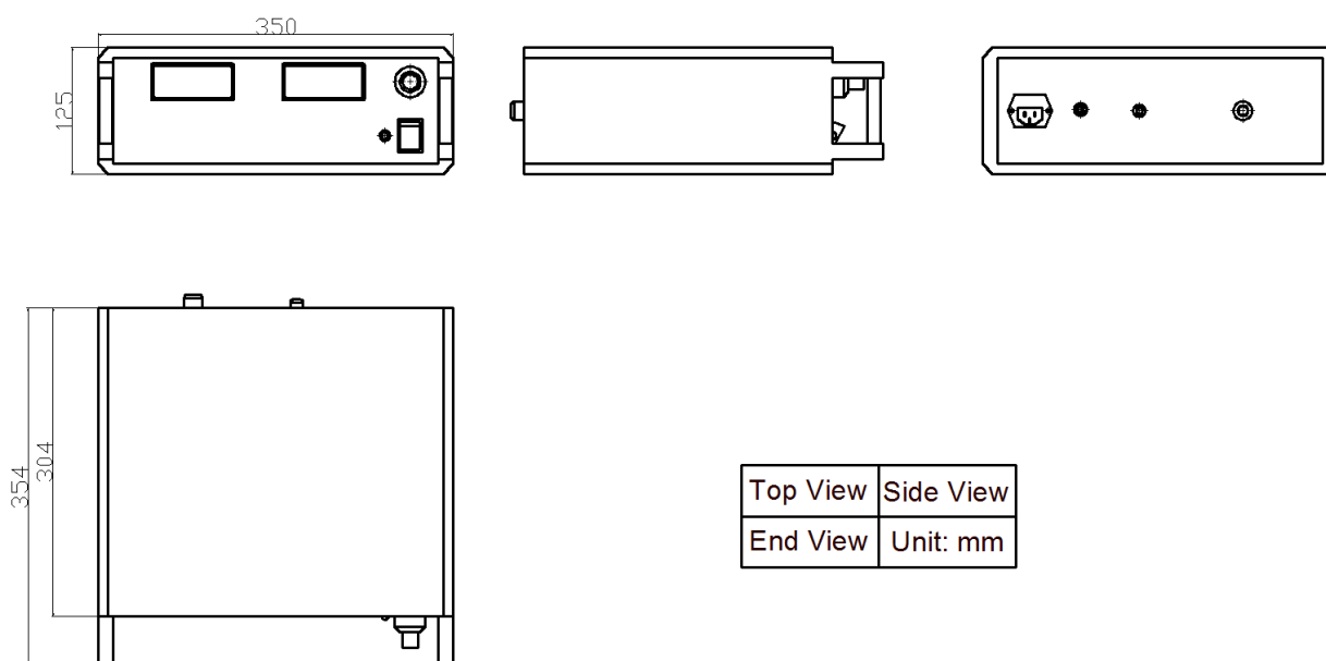
Figure 7. Dimensions for AHVACN20KV5MABT
