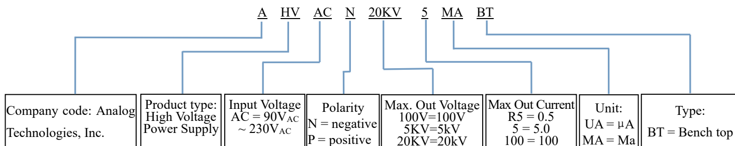
Figure 5. Naming Rules of AHVACN20KV5MABT
