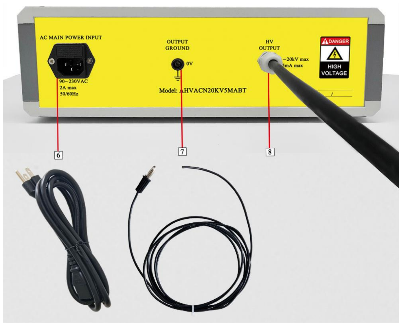
Figure 3. Front Panel
