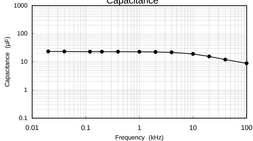
Capacitance
