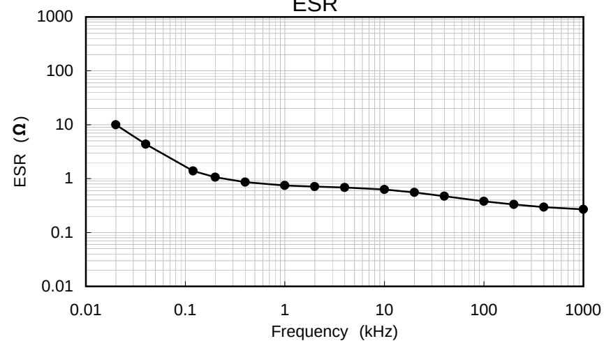
ESR
