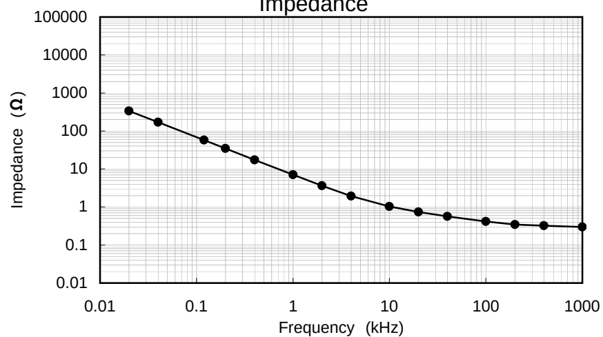
Impedance
