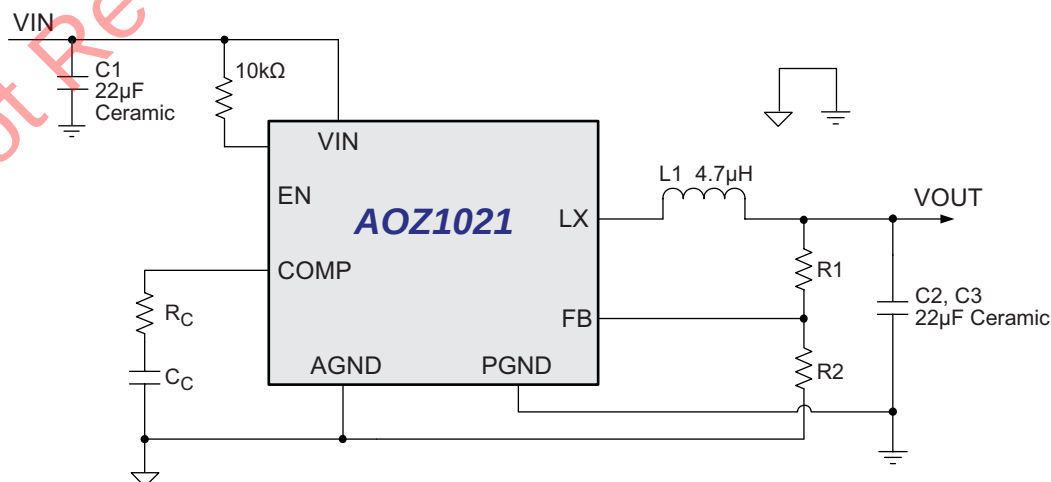
Figure 1. 3.3V/3A Buck Regulator
