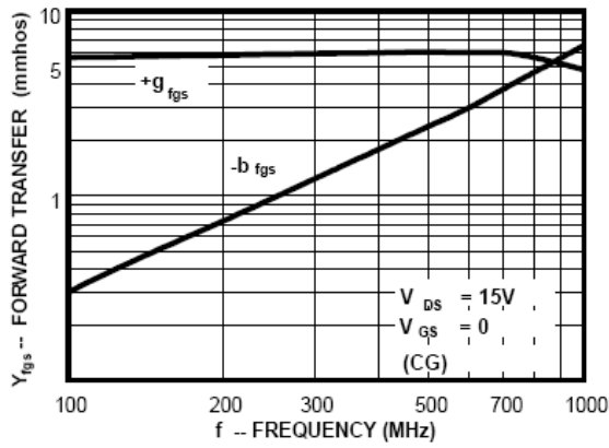
Figure 17. Forward Transadmittance
