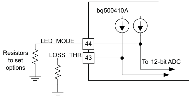
Figure 4. Option Programming
