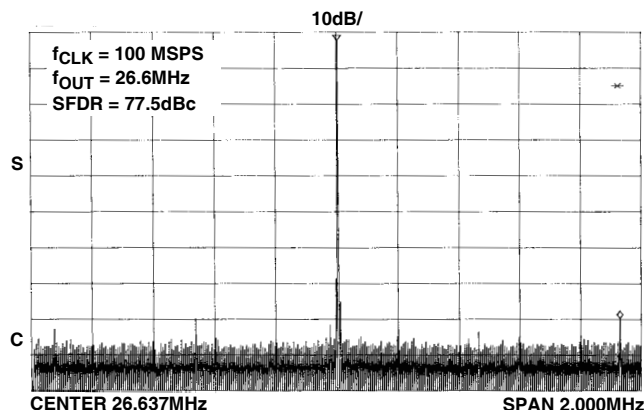
FIGURE 17. SFDR WITHIN A WINDOW
