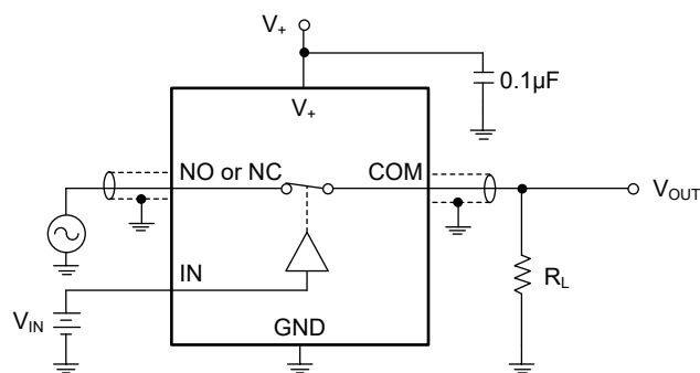
Test Circuit 8. Total Harmonic Distortion (THD)
