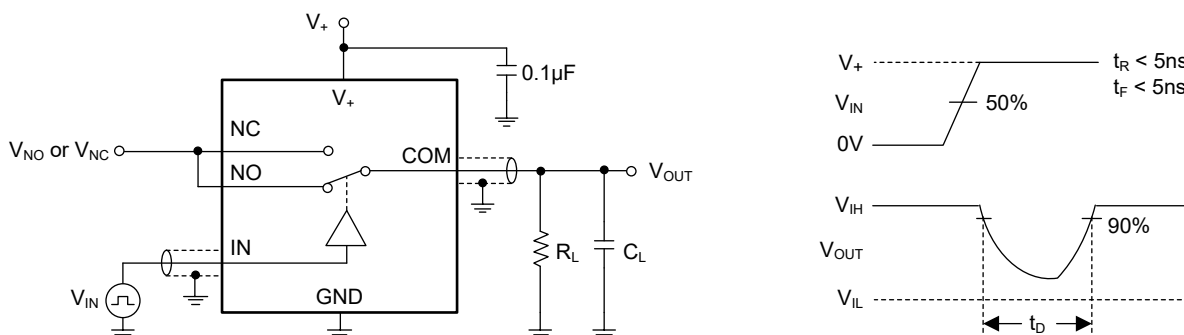
Test Circuit 3. Break-Before-Make Delay Time ( t_D )
