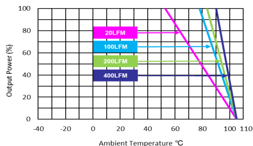
MKWI40-24S12, MKWI40-24S15 Derating Curve with Heatsink
