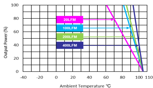
MKWI40-24S05, MKWI40-48S05, MKWI40-48S12, MKWI40-48S15 Derating Curve with Heatsink
