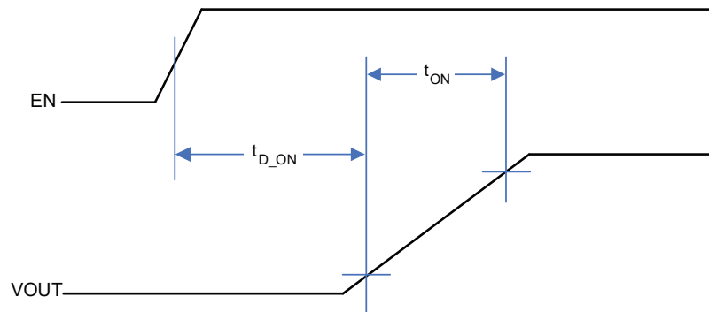
Figure 1. Turn-on Delay and Turn-on Time
