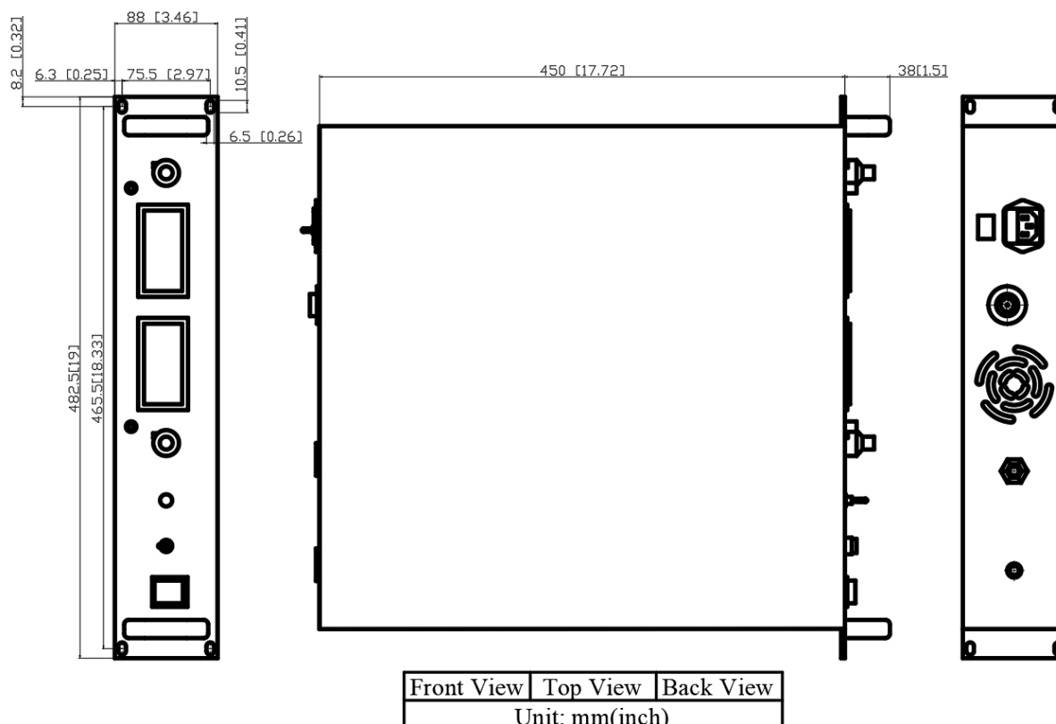
Figure 7. Dimensions for A2UHVACP30KV10MARM
