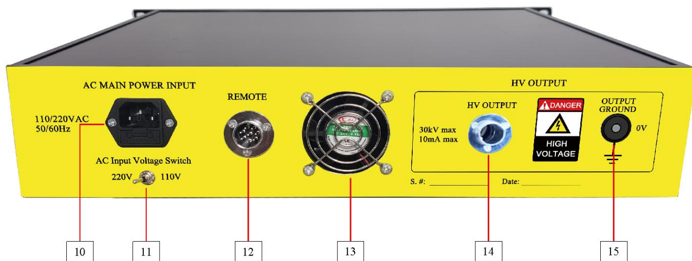
Figure 3. Front Panel
