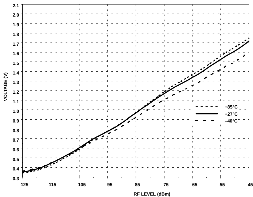
Figure 7. RSSI vs RF Level and Temperature - VCC = 3V
