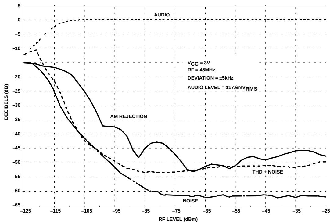
Figure 6. Sensitivity vs RF Level (+25°C)
