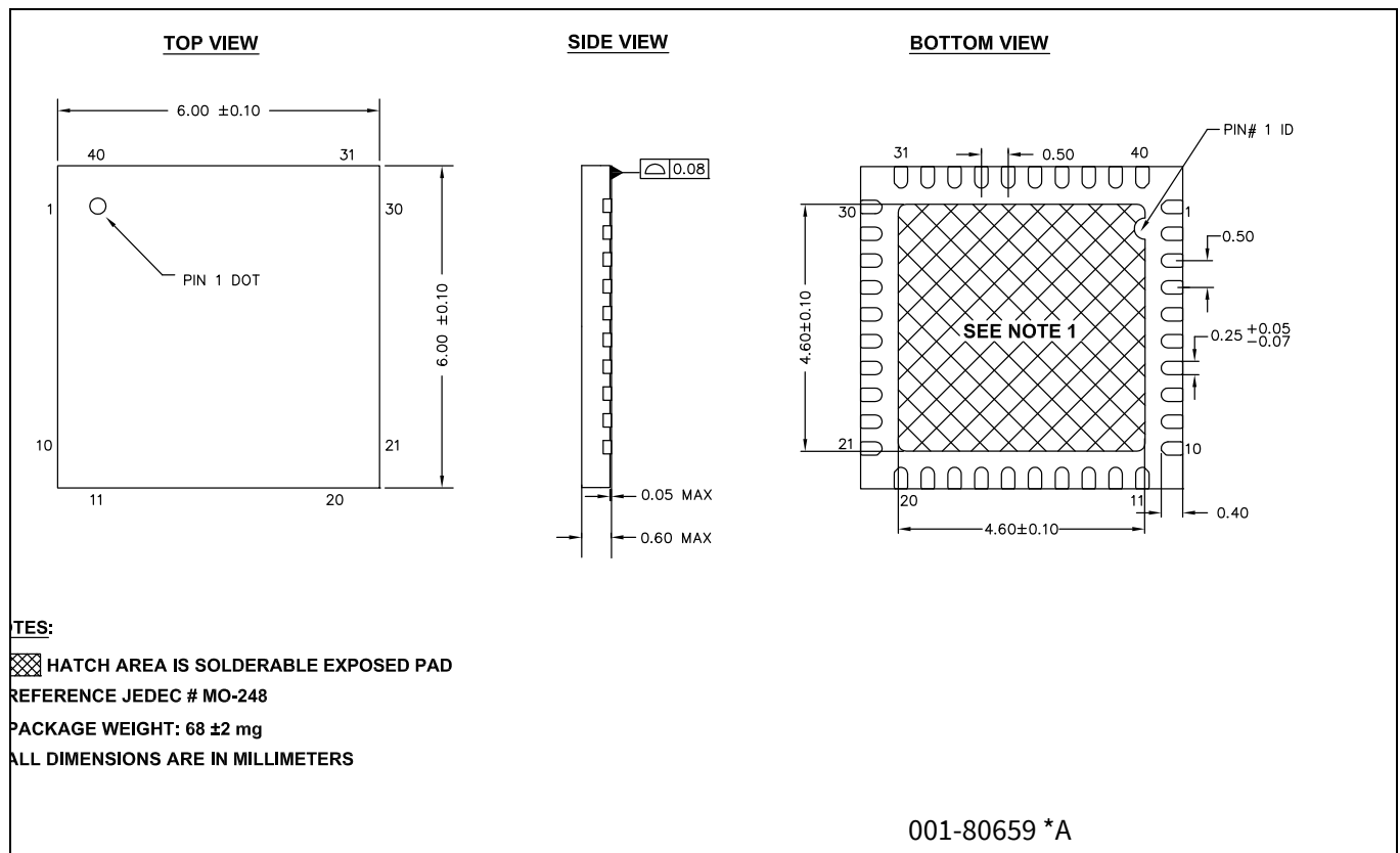
Figure 7 40L QFN 6×6×0.6 mm LR40A/LQ40A 4.6×4.6 E-PAD (SAWN), パッケージ外形, (PG-VQFN-40)
