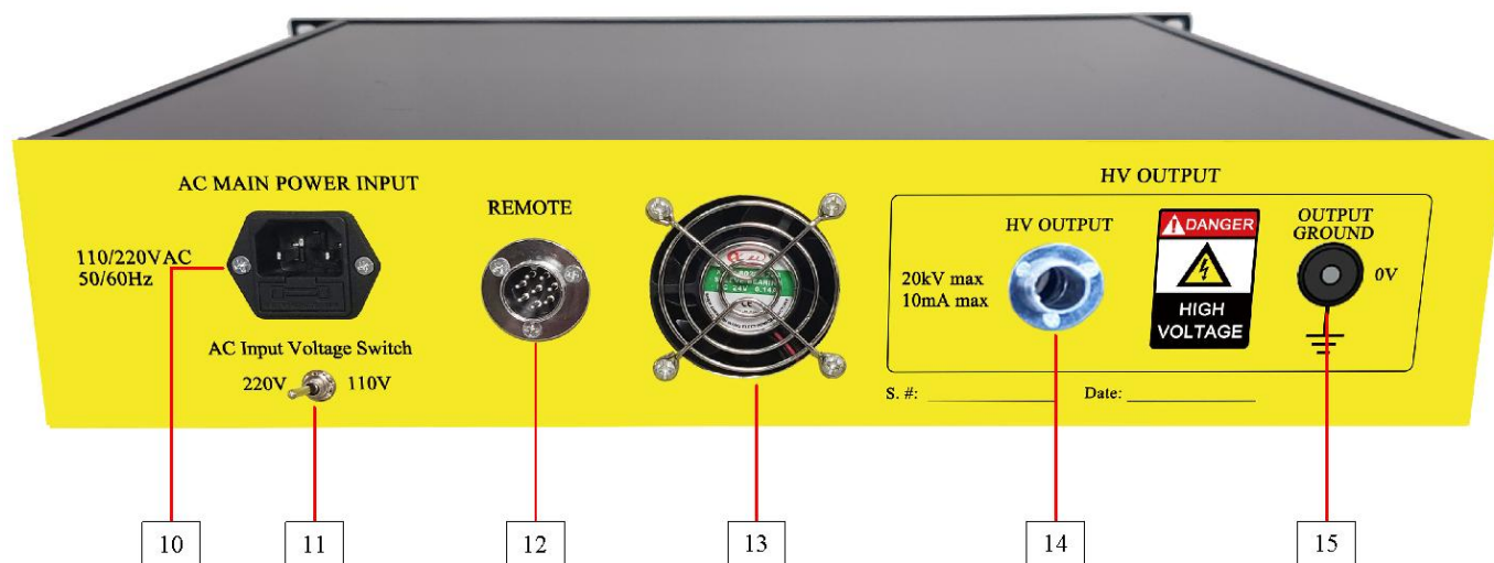
Figure 3. Front Panel
