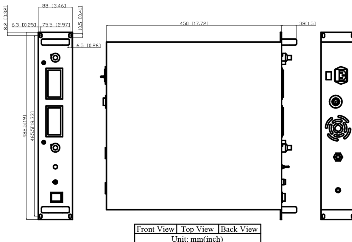
Figure 7. Dimensions for A2UHVACP20KV10MARM
