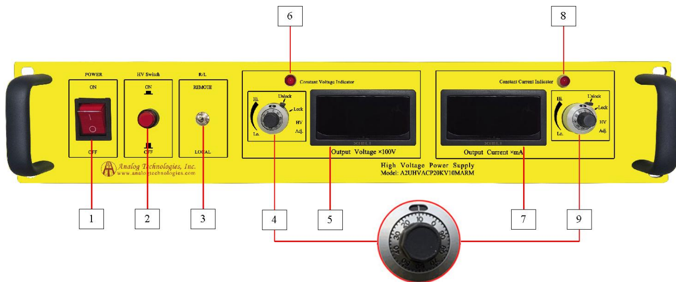
Figure 2. Front Panel
