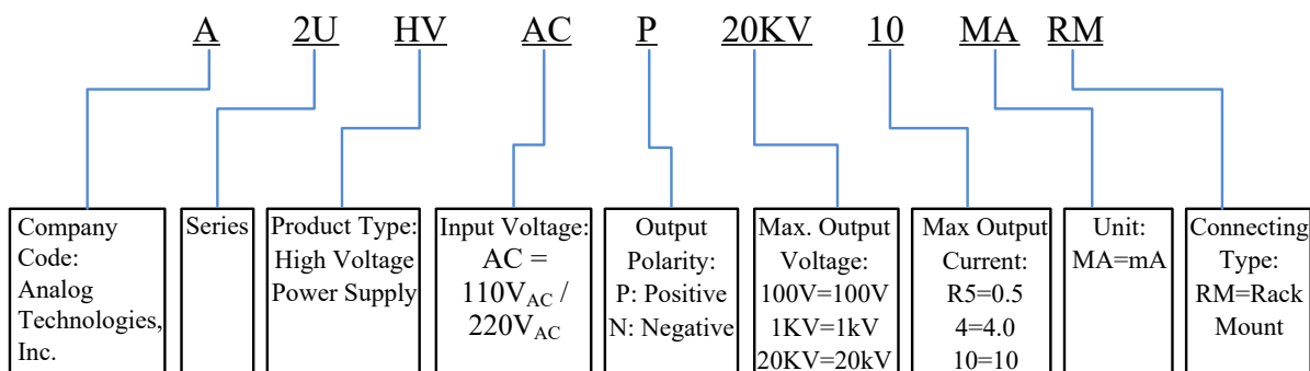
Figure 5. Naming Rules of A2UHVACP20KV10MARM
