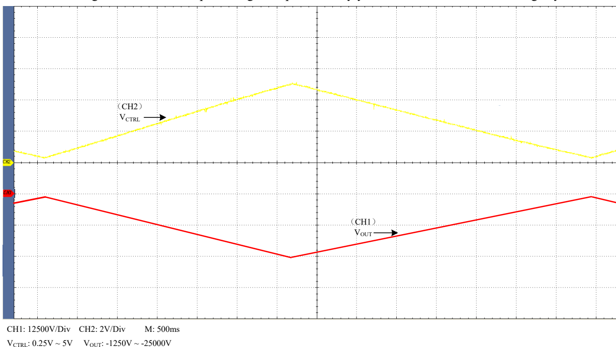
Figure 3. Triangle Wave
