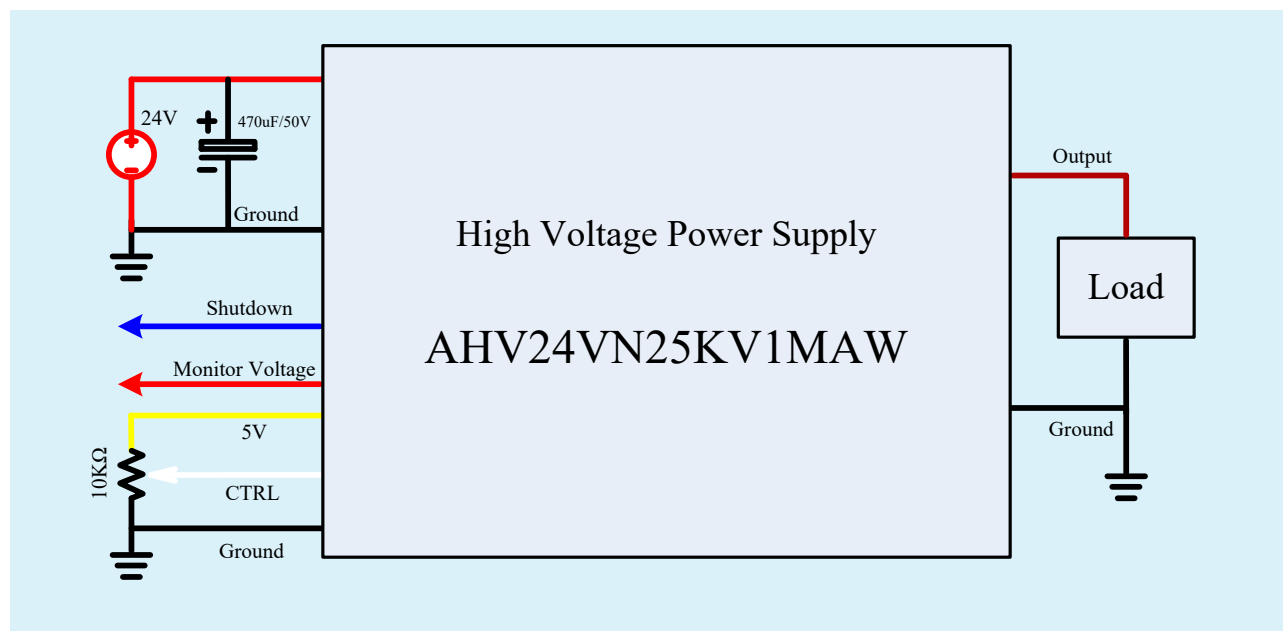
Figure 8. Figure 8. Control by External Signal Source
