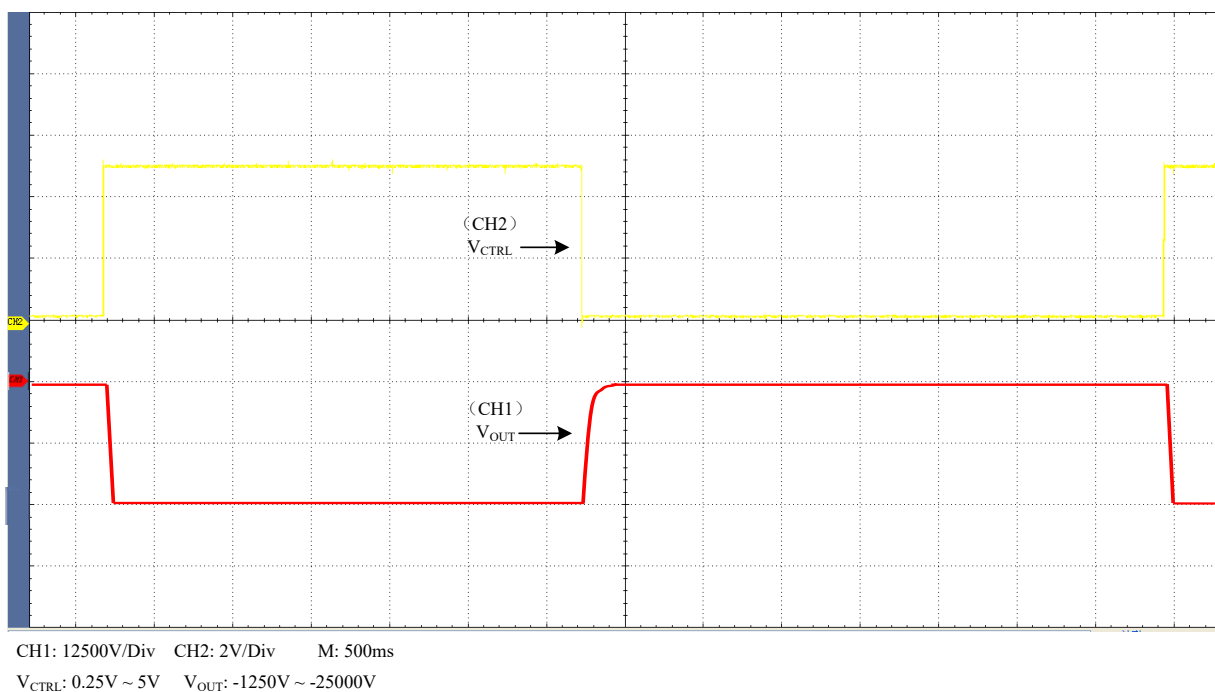
Figure 5. Square Wave
