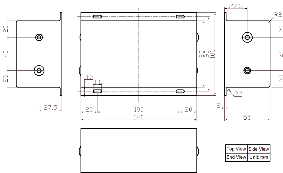
Figure 11. Dimensions for AHV24VN25KV1MAW
