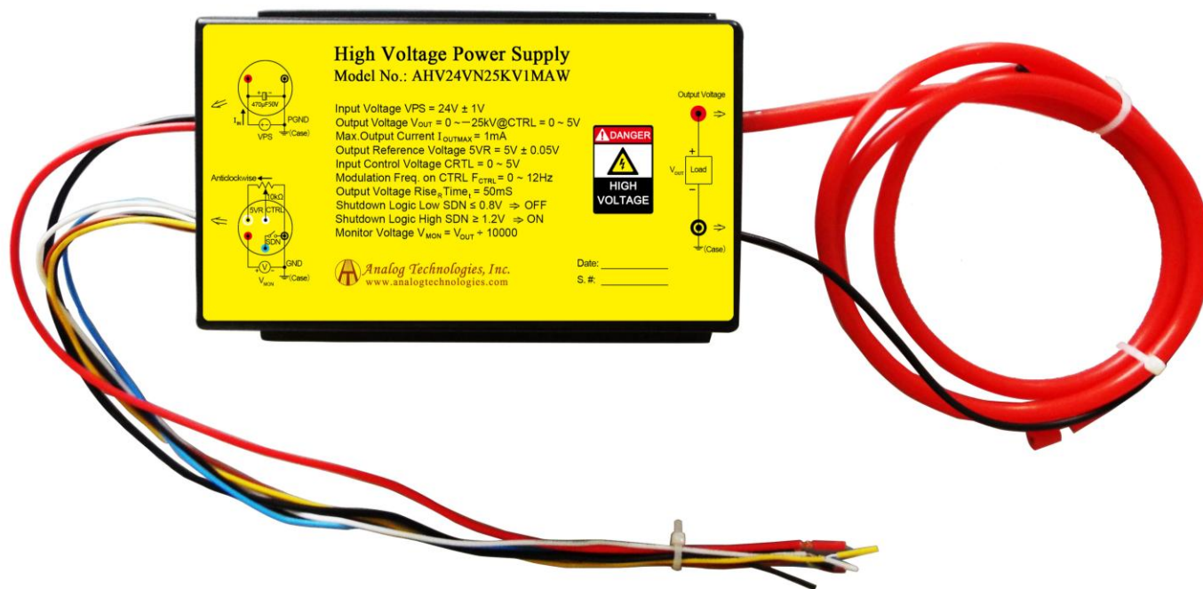
Figure 10. Leads of AHV24VN25KV1MAW
