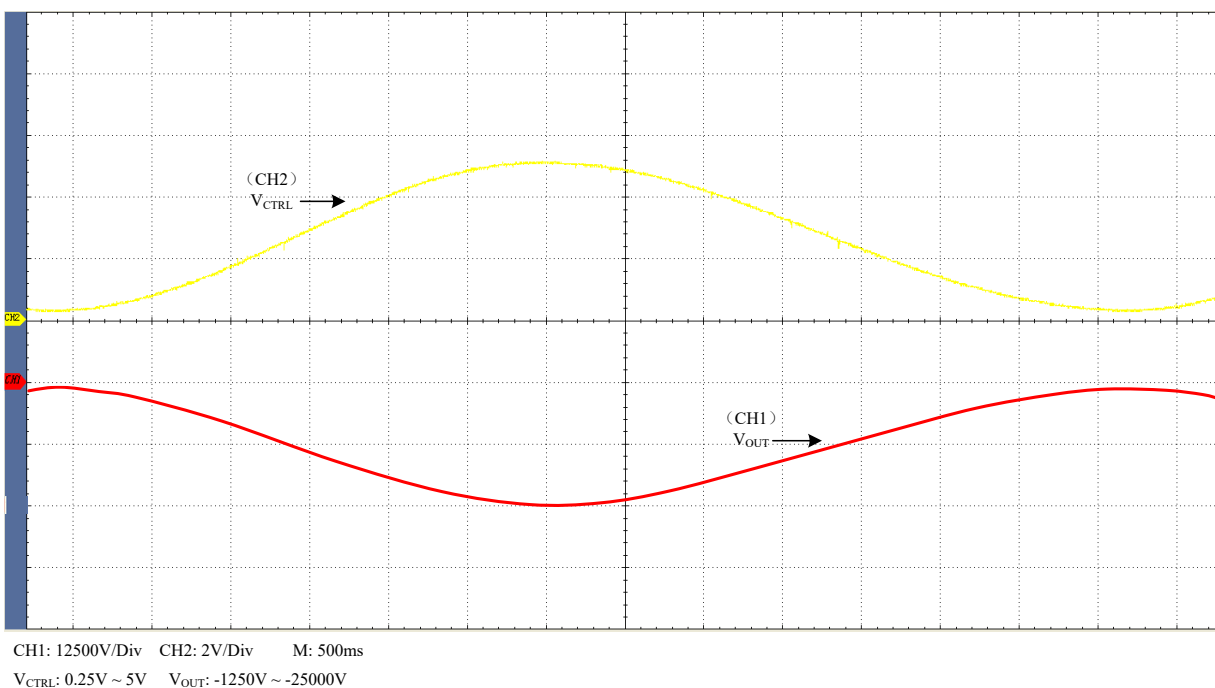
Figure 4. Sine Wave
