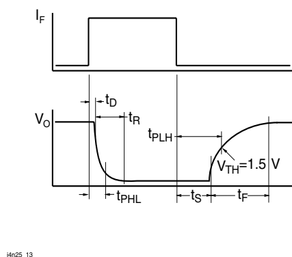
Figure 13. Switching Timing
