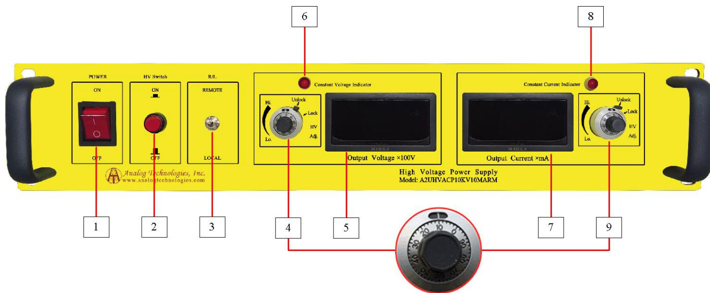
Figure 2. Front Panel
