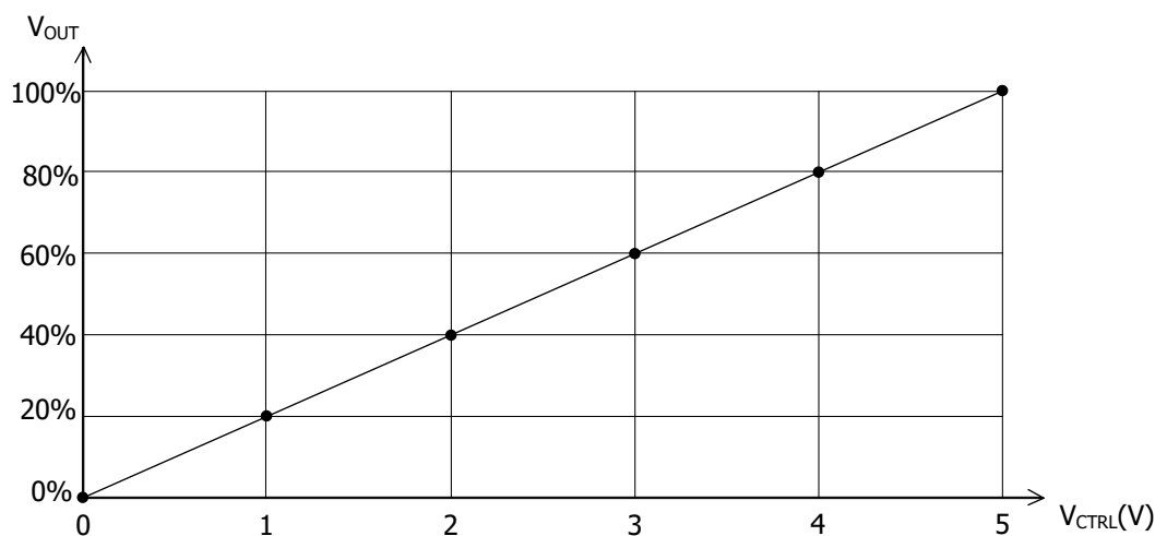
Figure 6. V_{CTRL} vs. V_{VOUT}
