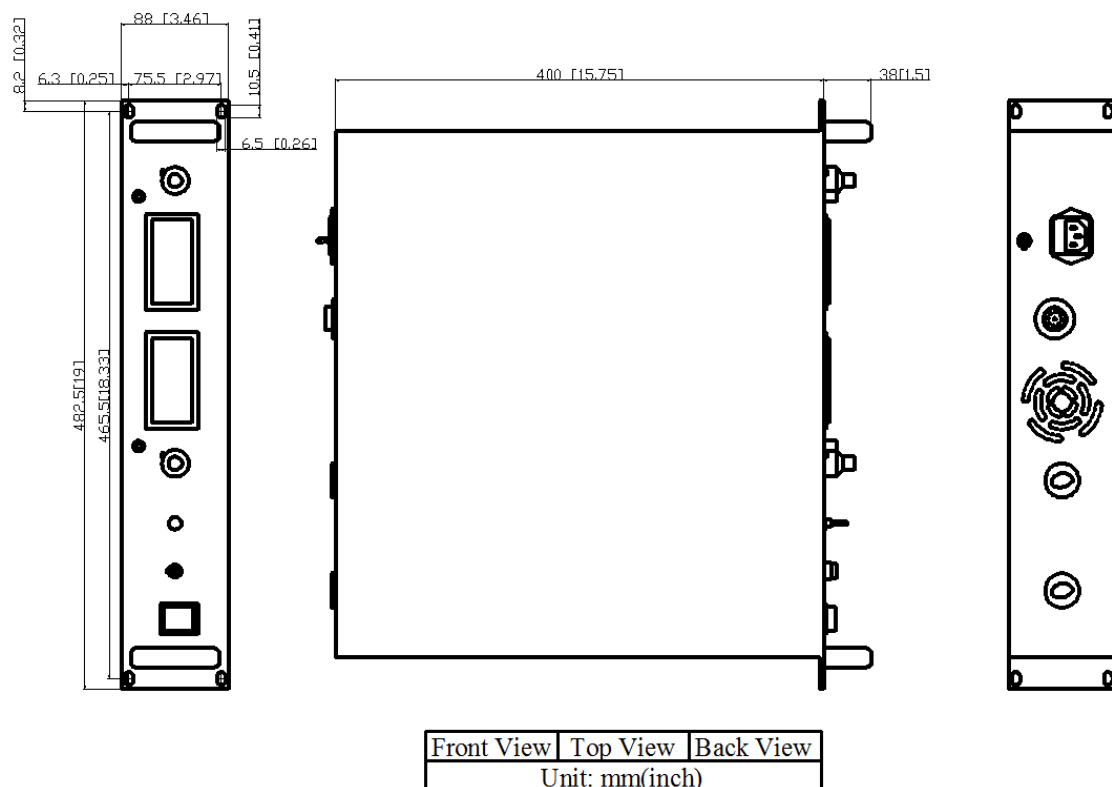
Figure 7. Dimensions for A2UHVACP10KV10MARM
