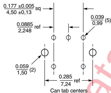
Recommended Board Layout
