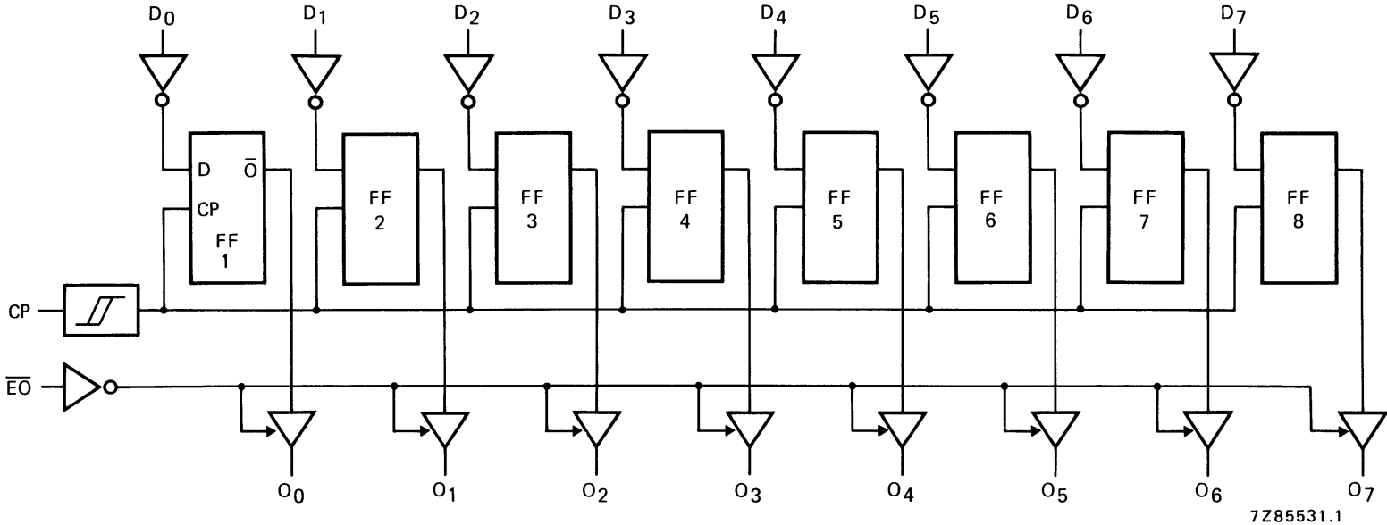
Fig.3 Logic diagram.
