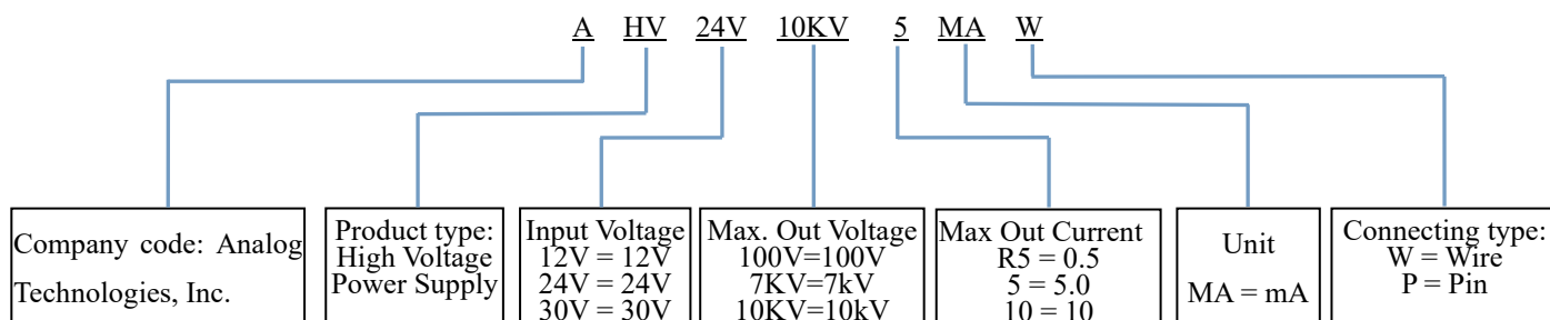
Figure 10. Naming Rules of AHV24V10KV5MAW
