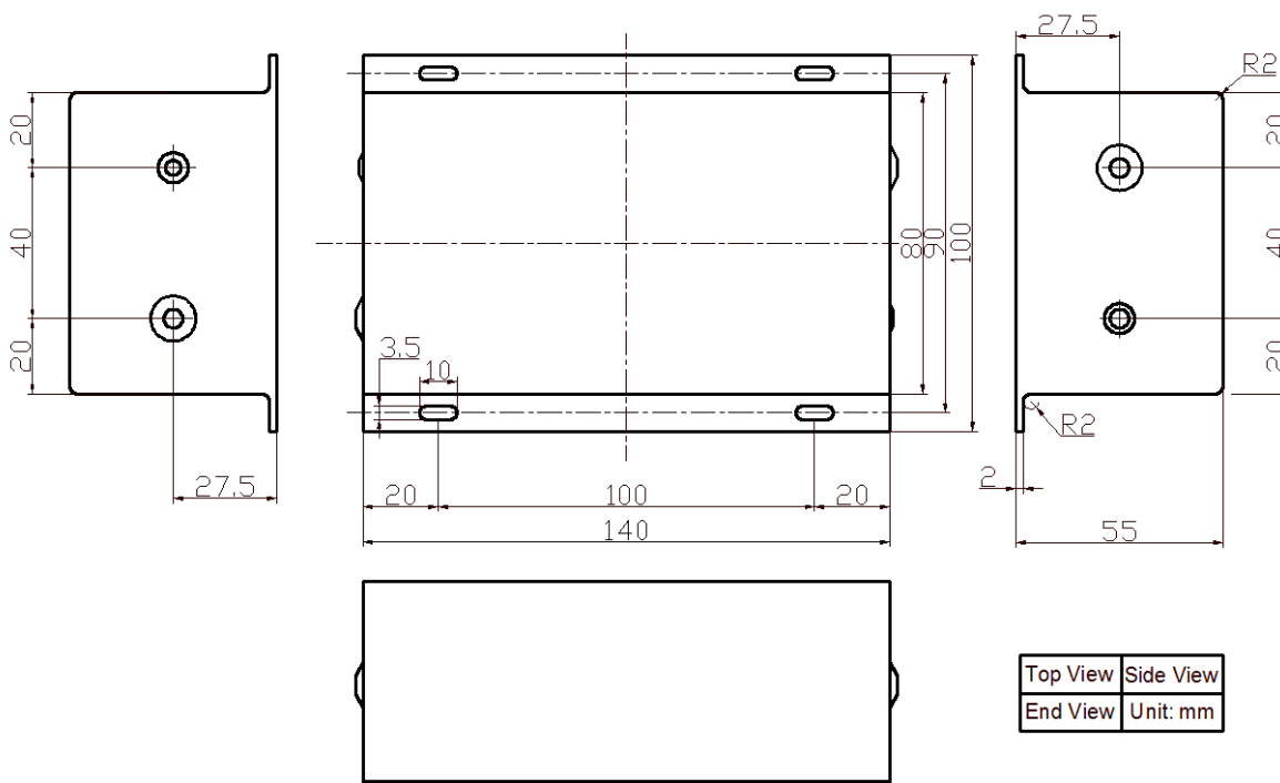
Figure 12. Dimensions for AHV24V10KV5MAW
