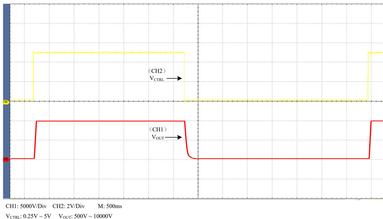
Figure 5. Square Wave
