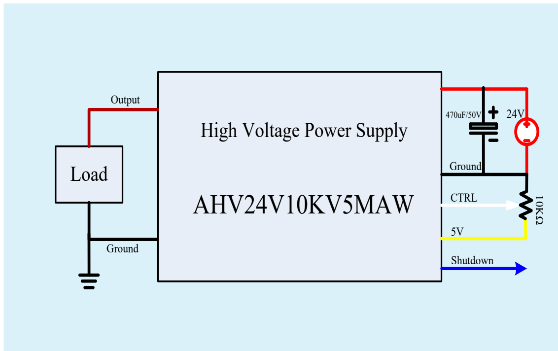
Figure 8. Control by External Signal Source
