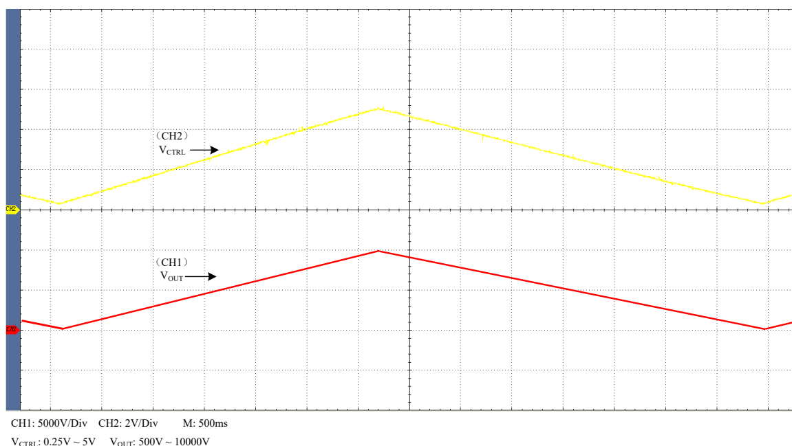
Figure 3. Triangle Wave
