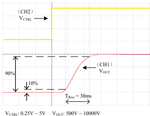
Figure 6. Rise Time
