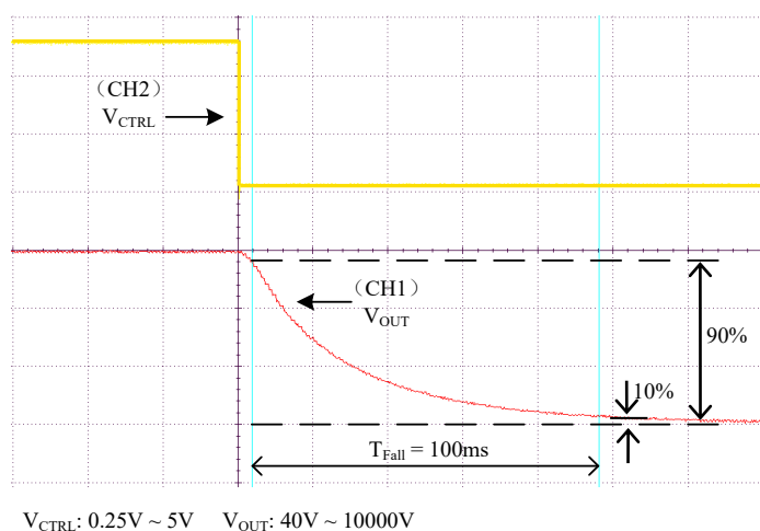
Figure 7. Fall Time
