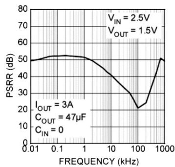
FIGURE 2-1: Power Supply Rejection Ratio.
