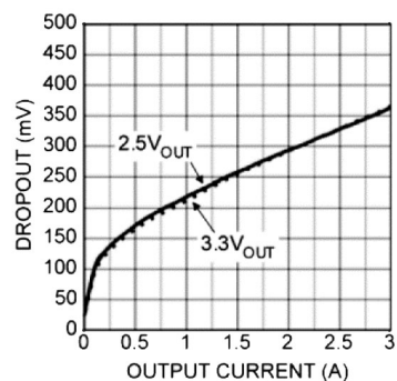
FIGURE 2-3: Dropout vs. Output Current.
