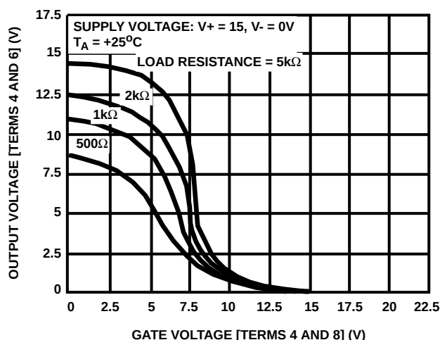
FIGURE 5. VOLTAGE TRANSFER CHARACTERISTICS OF CMOS OUTPUT STAGE
