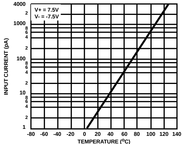
FIGURE 11. INPUT CURRENT vs AMBIENT TEMPERATURE
