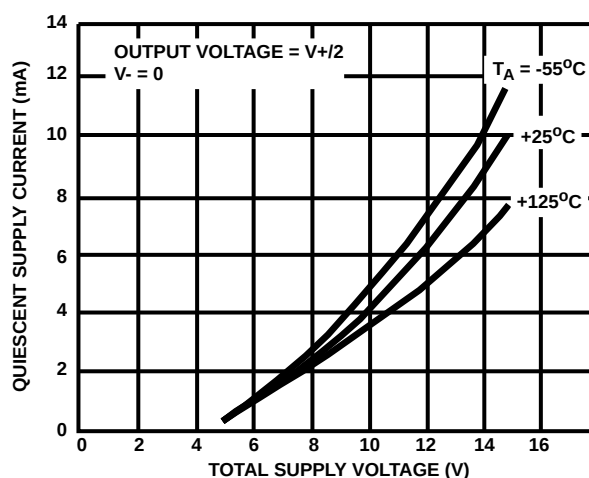
FIGURE 7. QUIESCENT SUPPLY CURRENT vs SUPPLY VOLTAGE
