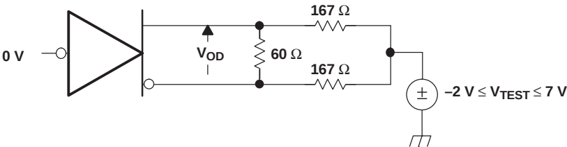
Figure 2. Driver V_{\text{OD}}
