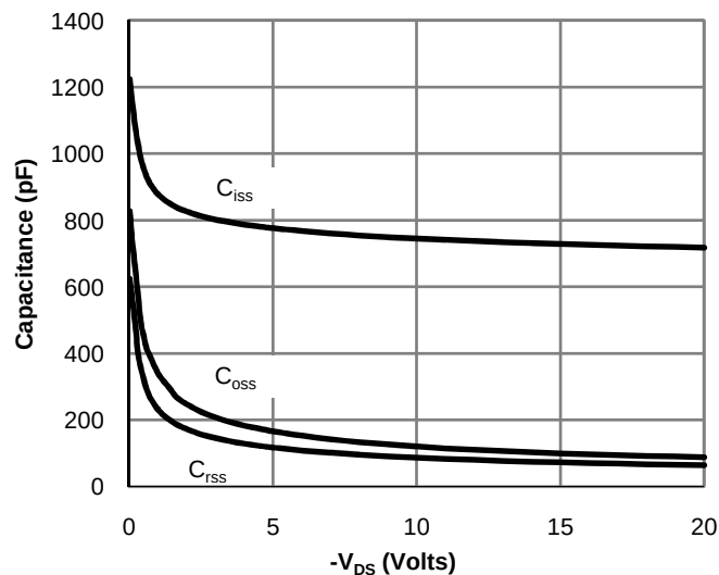
Figure 8: Capacitance Characteristics
