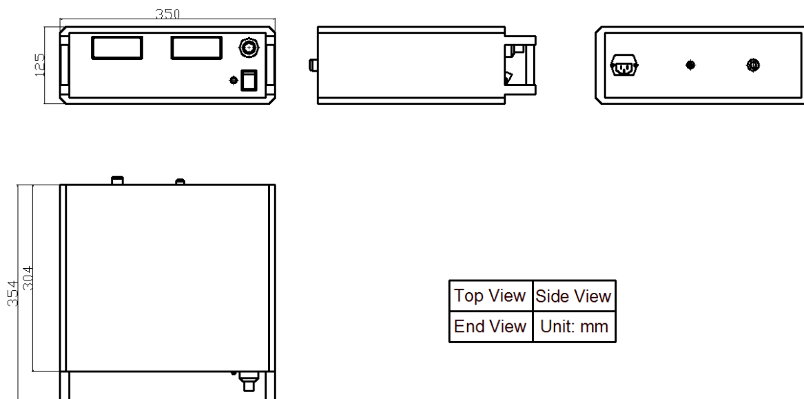
Figure 7. Dimensions for AHVACN50KVR5MABT
