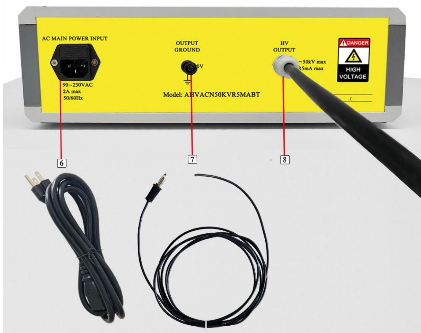
Figure 3. Back Panel
