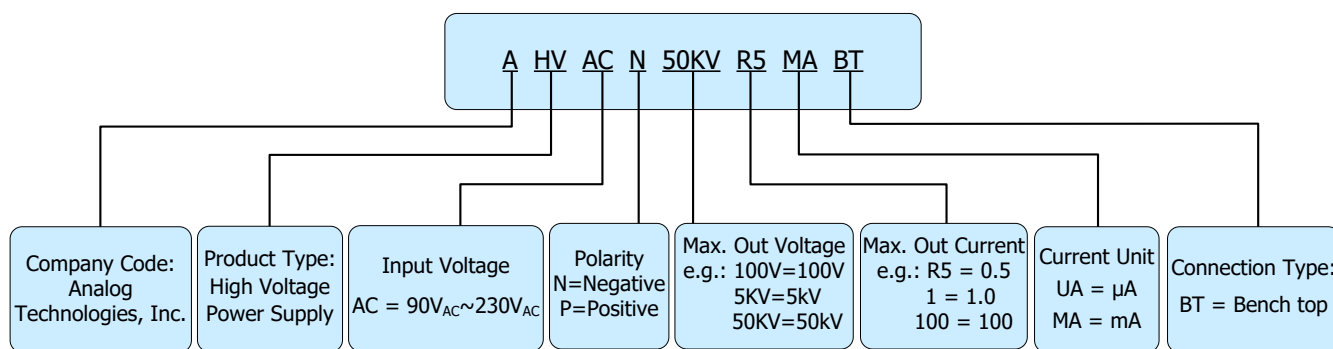
Figure 5. Naming Rules of AHVACN50KVR5MABT
