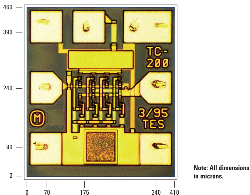
Figure 5. Bonding pad locations
