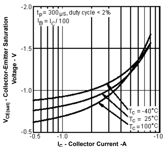
Collector-Emitter Saturation Voltage vs Collector Current
