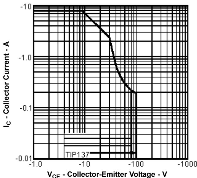
Maximum Forward-Bias Safe Operating Area
