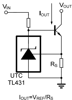
Constant-current Sink
