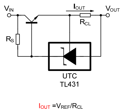
Current Limiting or Current Source
