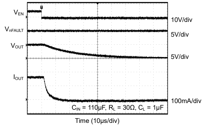
Turn-Off Response (SGM2588A/C/E/G/I/K)
