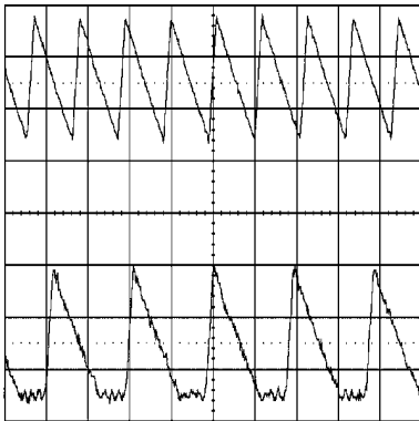
CCM and DCM Operating Modes V_{IN} = 24V , V_O = 3.3V , I_O = 3A/0.4A 2 \mu sec/div
