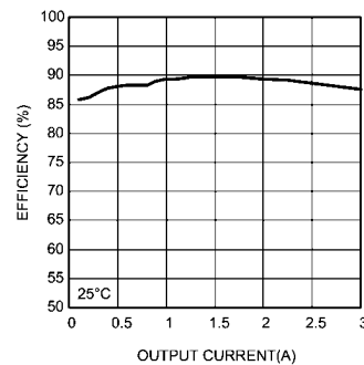
Efficiency V_{IN} = 24\text{V} V_{OUT} = 5.0\text{V}
