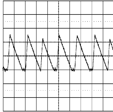
Transition Mode Operation V_{IN} = 24V , V_O = 3.3V , I_O = 0.5 A 2 \mu sec/div
