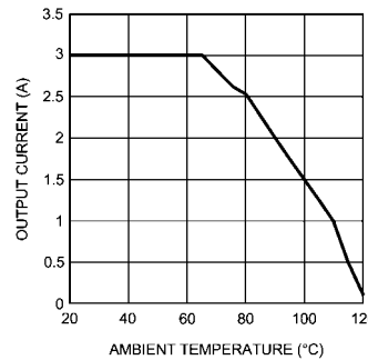
Thermal Derating Curve V_{IN} = 24\text{V} , V_{OUT} = 5.0\text{V} ,
