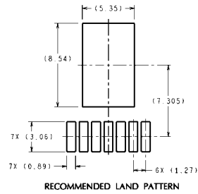
7-Lead TZA Package NS Package Number TZA07A
