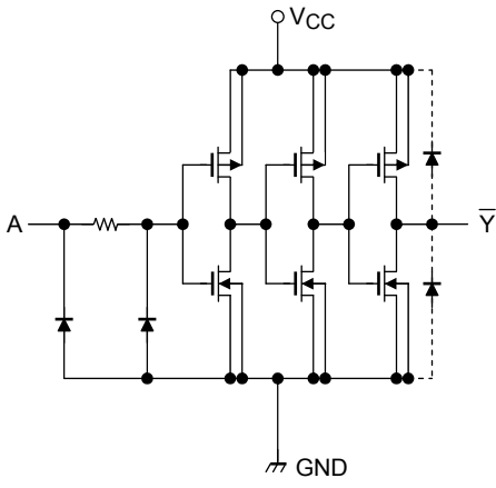
TC74HC4049A
