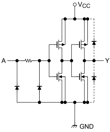
TC74HC4050A
