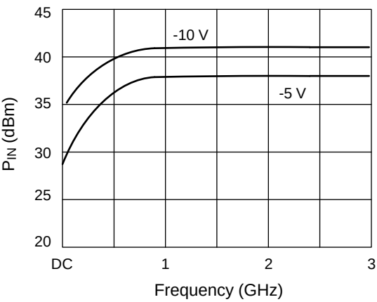
PIN at 1 dB Compression vs. Frequency and Control Voltage
