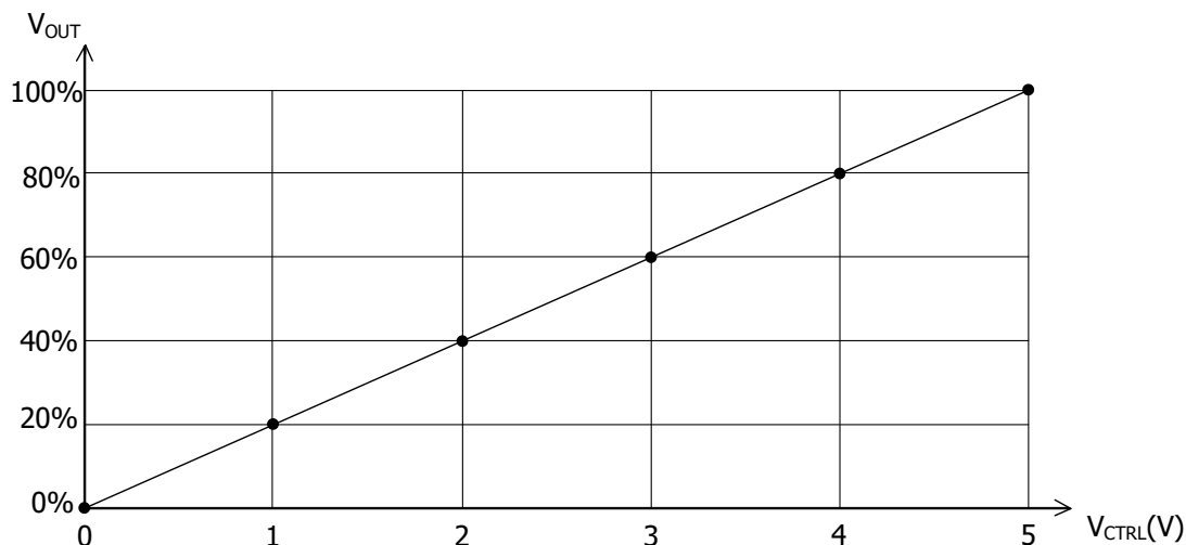
Figure 5. V_CTRL vs. V_OUT
