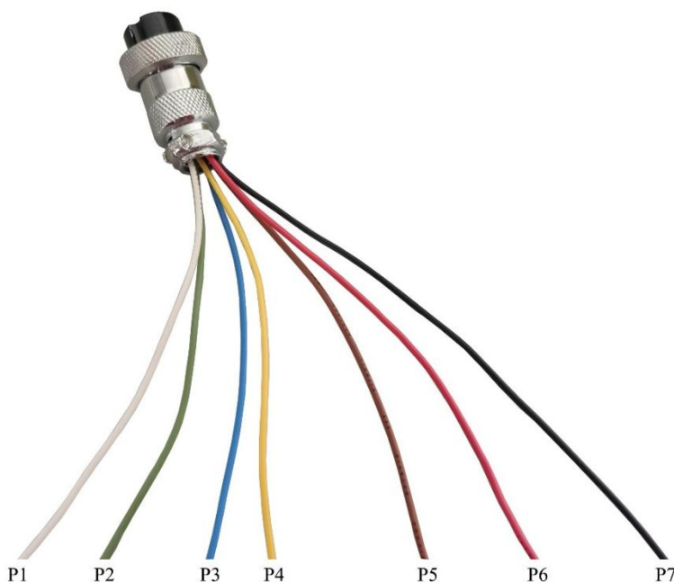
Figure 4. 8-pin Connector
