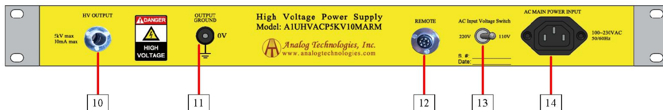
Figure 3. Front Panel
