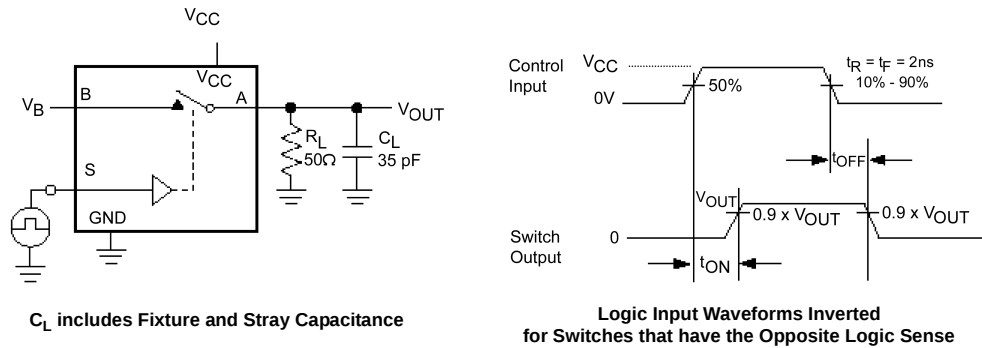
FIGURE 1. Turn-On/Turn-Off Timing
