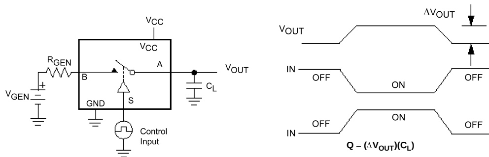
FIGURE 4. Charge Injection
