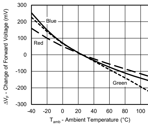
Fig. 7 - Change of Forward Voltage vs. Ambient Temperature
