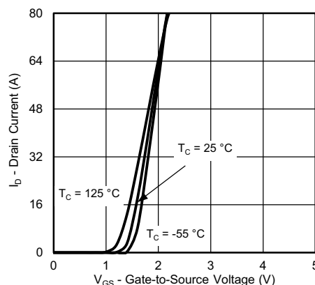
Transfer Characteristics
