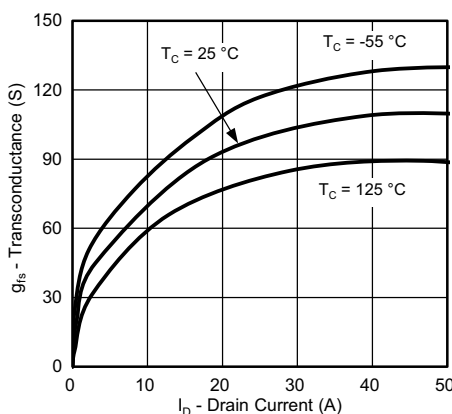
Transconductance
