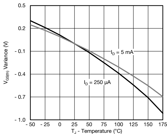
Threshold Voltage
