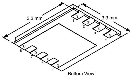
PowerPAK® 1212-8
