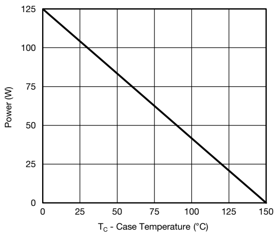
Power, Junction-to-Case
